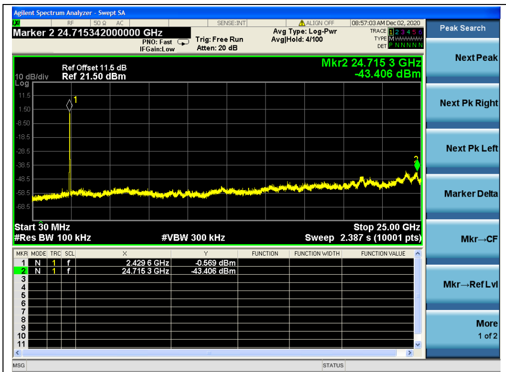
(30MHz to 25GHz, Channel 7, 802.11n (HT40))
