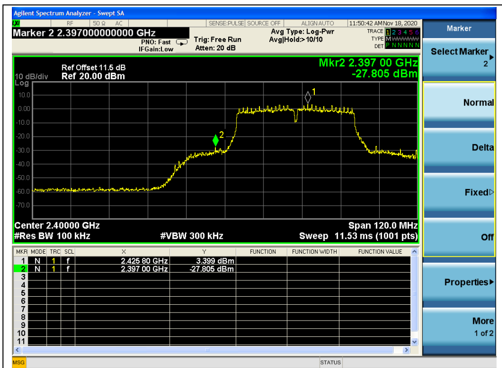
(Band Edge, Channel 3, 802.11n (HT40))
