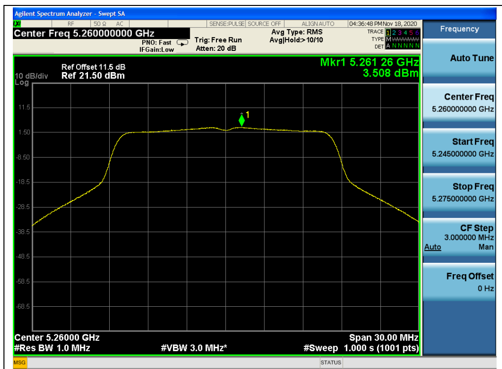
(Channel 52, 5260MHz, 802.11a, ANT1)
