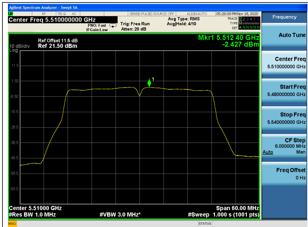
(Channel 102, 5510MHz, 802.11n (HT40), ANT1)
