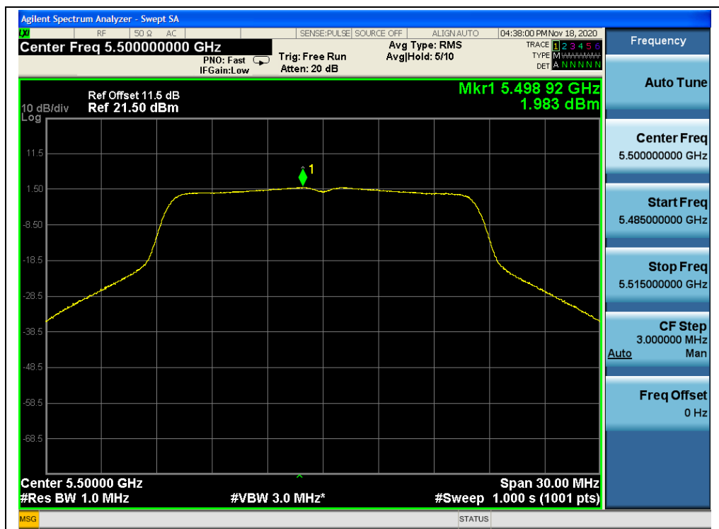
(Channel 100, 5500MHz, 802.11a, ANT1)
