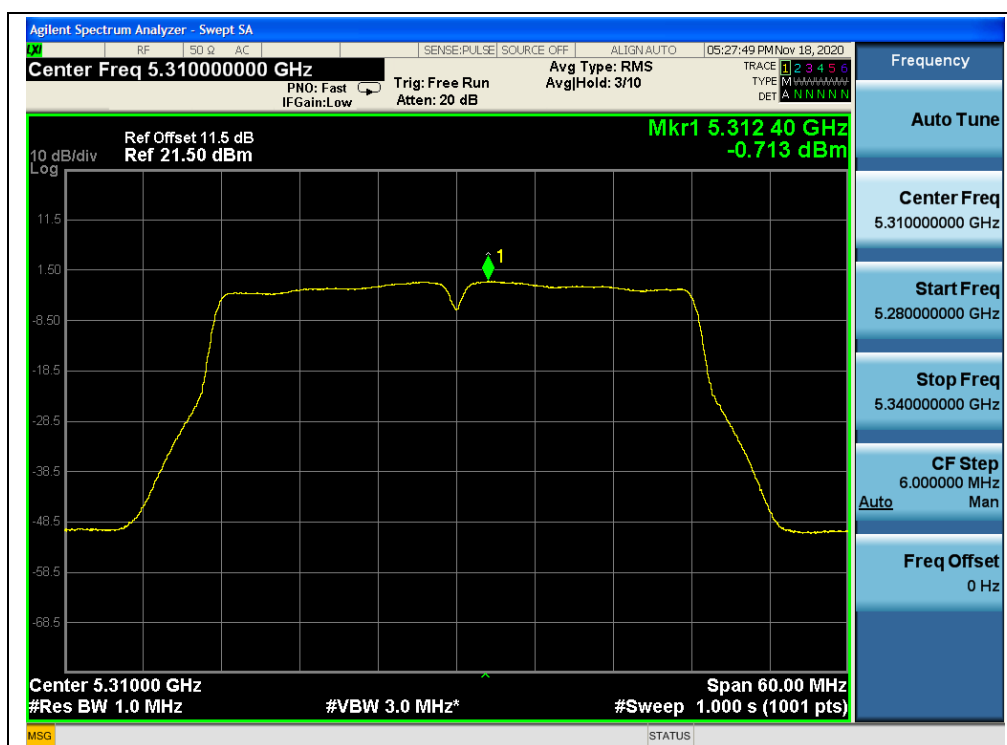
(Channel 62, 5310MHz, 802.11n (HT40), ANT1)
