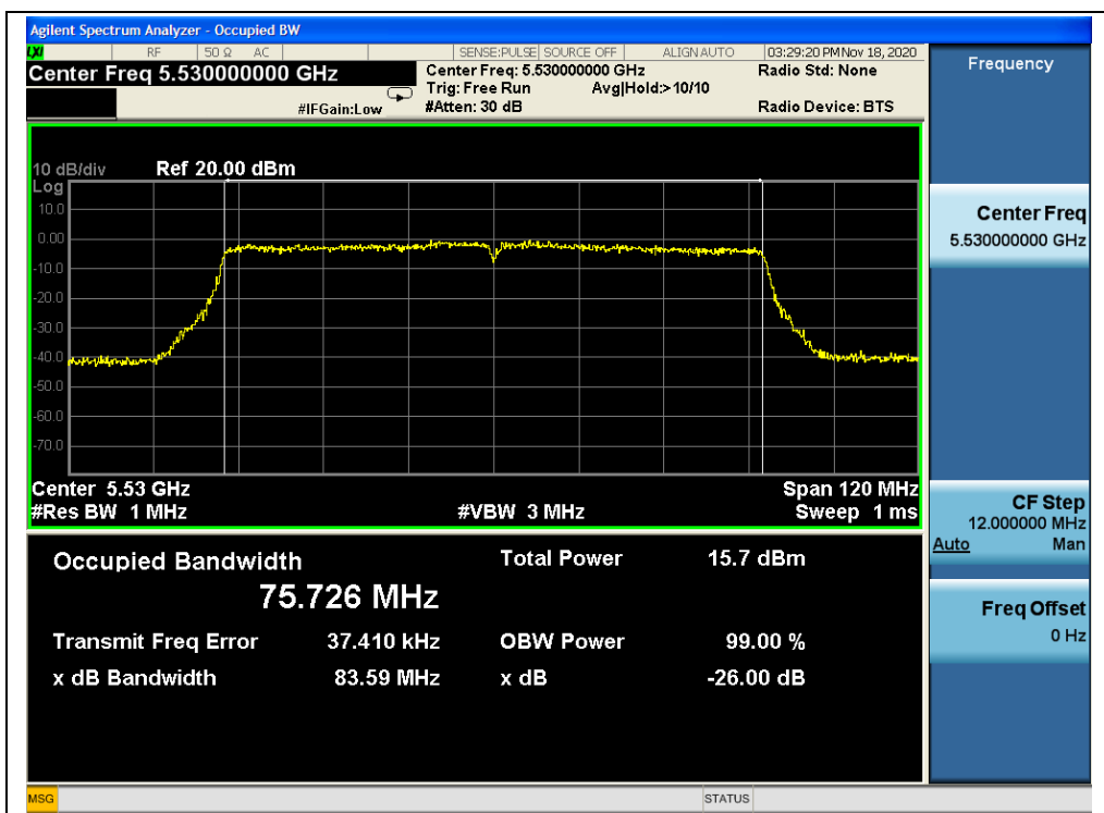
(Channel 106, 5530MHz, 802.11ac (VHT80))
