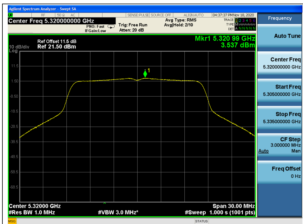
(Channel 64, 5320MHz, 802.11a, ANT1)
