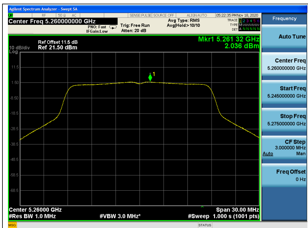
(Channel 52, 5260MHz, 802.11n (HT20), ANT1)
