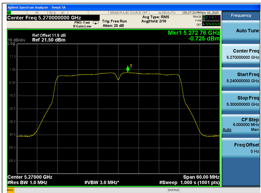
(Channel 54, 5270MHz, 802.11n (HT40), ANT1)
