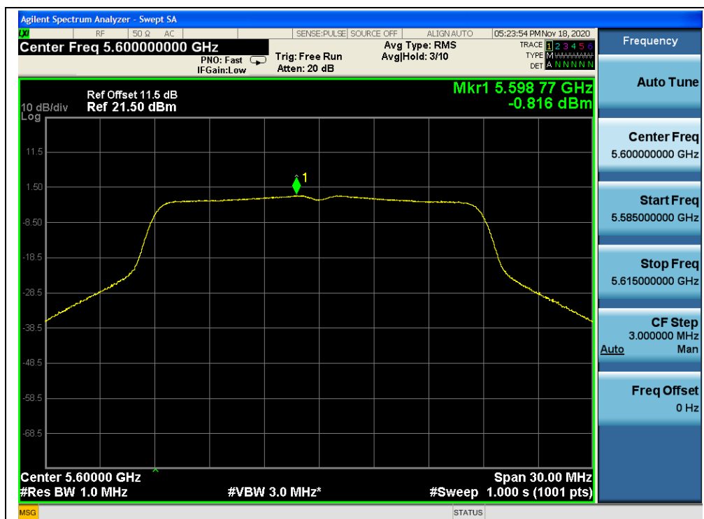
(Channel 120, 5600MHz, 802.11n (HT20), ANT1)
