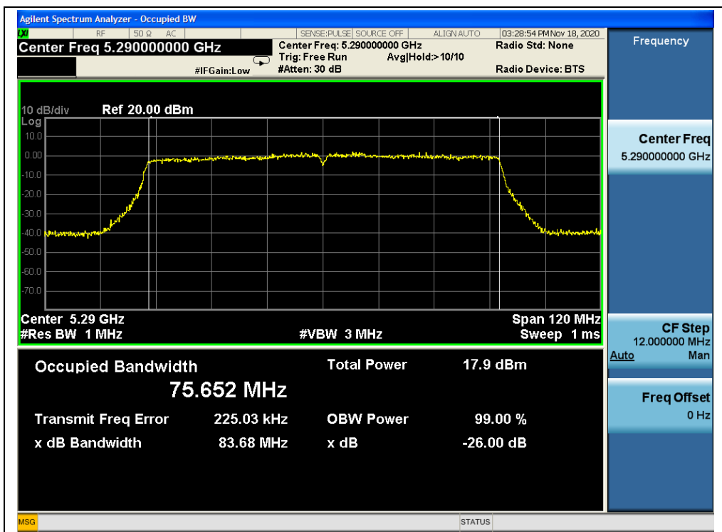
(Channel 58, 5290MHz, 802.11ac (VHT80))
