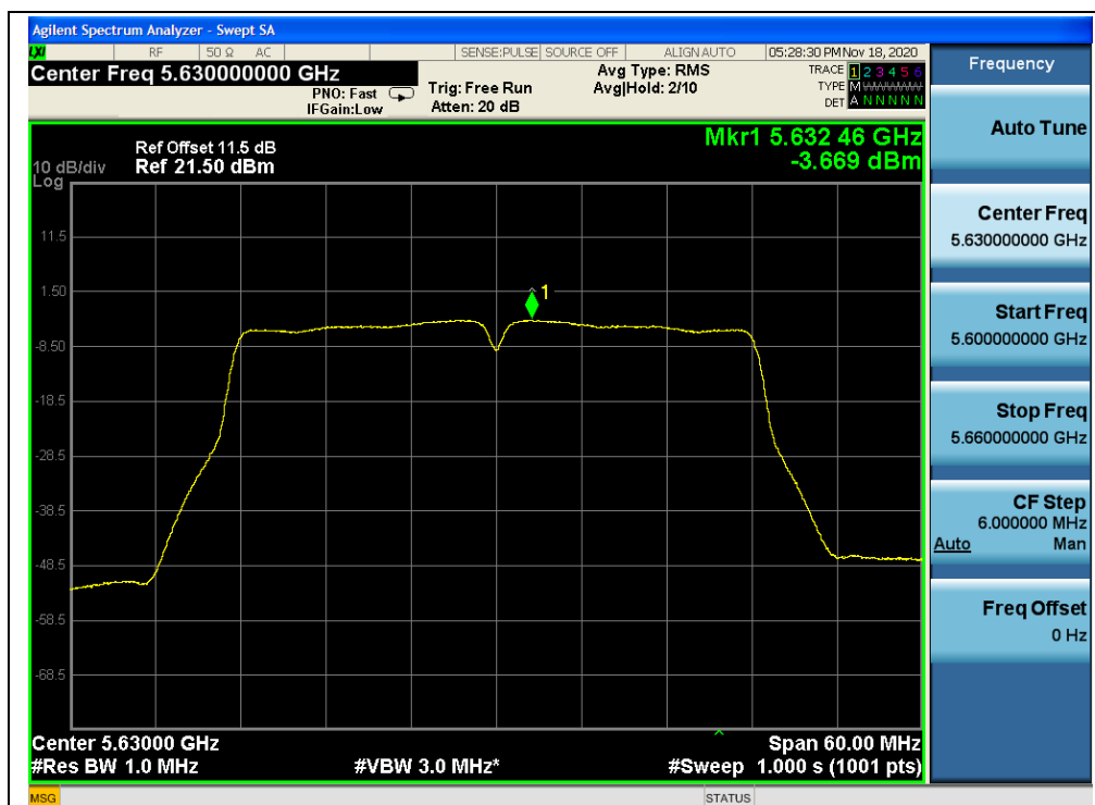
(Channel 126, 5630 MHz, 802.11n (HT40), ANT1)
