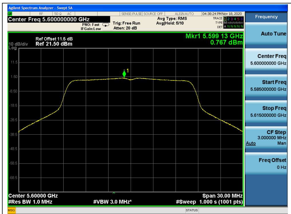
(Channel 120, 5600MHz, 802.11a, ANT1)
