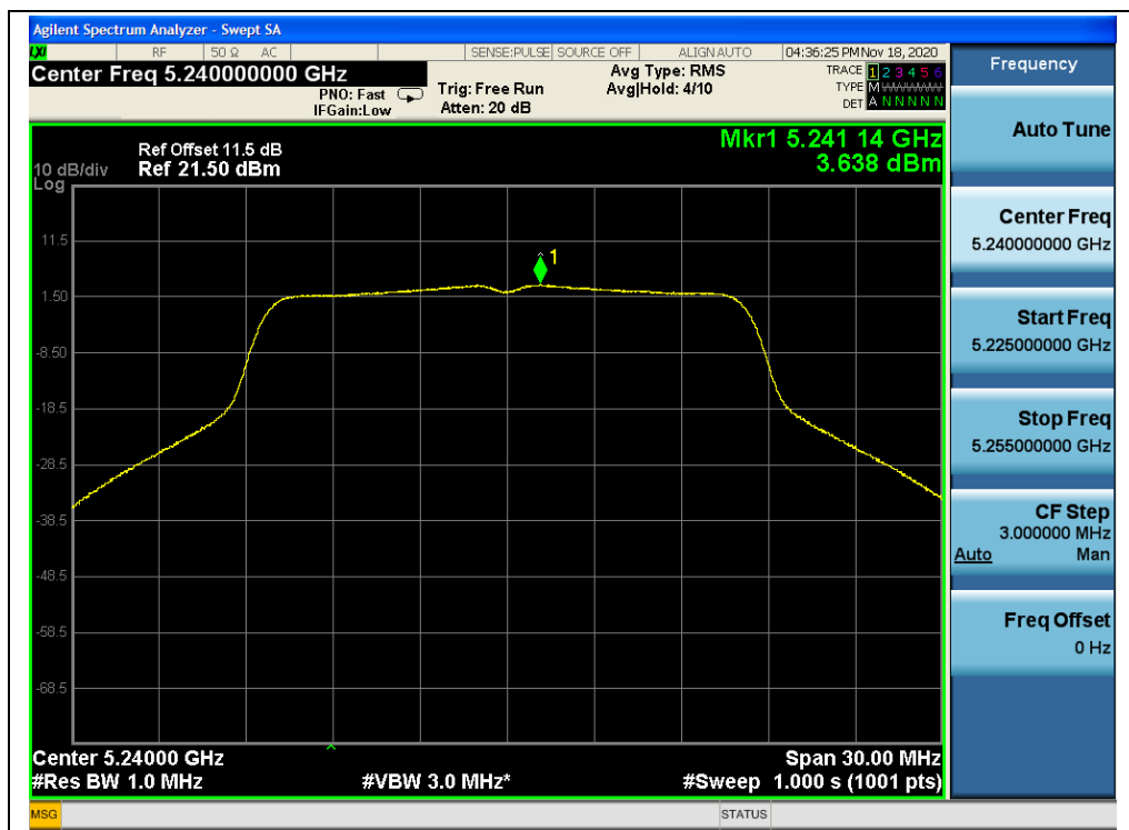
(Channel 48, 5240MHz, 802.11a, ANT1)
