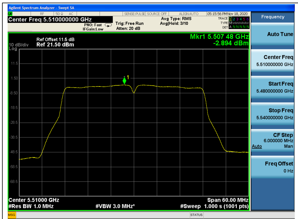
(Channel 102, 5510MHz, 802.11ac (VHT40), ANT1)
