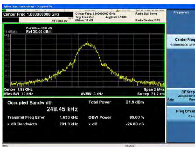
GSM1900(EDGE), CH661, 1880.0MHz
