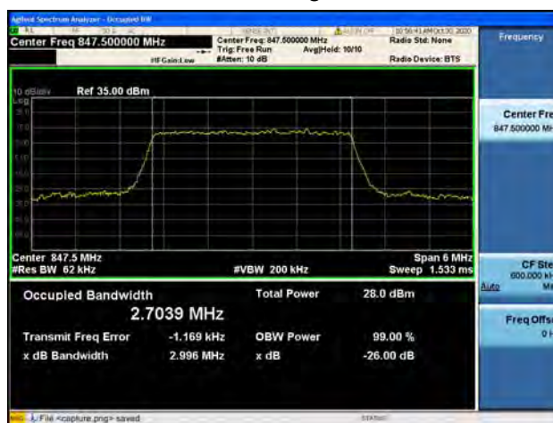
Band5 / 3MHz / High CH / 64QAM
