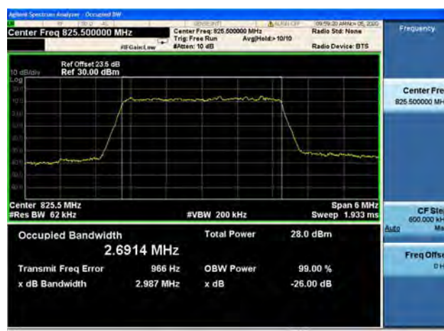
Band26 / 3MHz / Low CH / 64QAM
