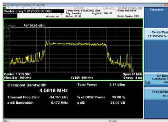
B12_N25(5M)_CP-OFDM_QPSK_High CH
