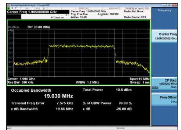
B12_N25(20M)_CP-OFDM_QPSK_high CH
