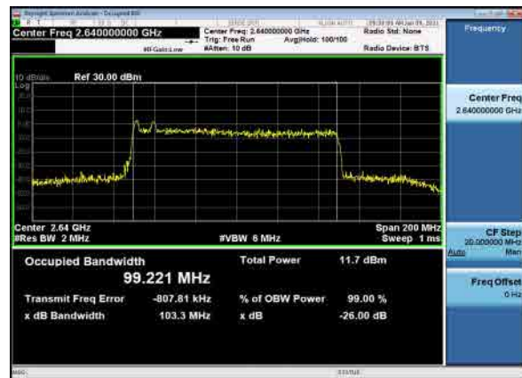
B26_N41(100M)_CP-OFDM_QPSK_high_OBW
