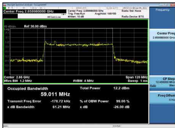
B26_N41(60M)_DFT-s-OFDM_64 QAM_high_OBW
