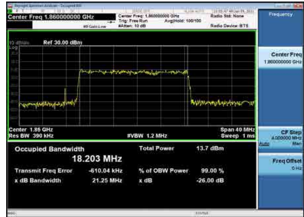
B12_N25(20M)_DFT-s-OFDM_QPSK_Low CH
