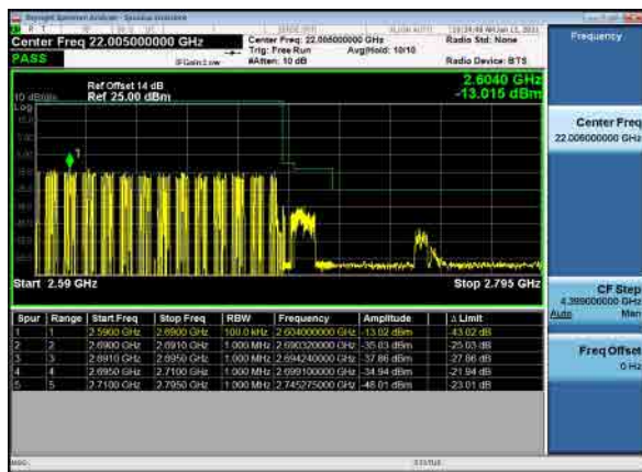
B26_N41(100M)_DFT-s-OFDM_BPSK_Full RB_High_CH
