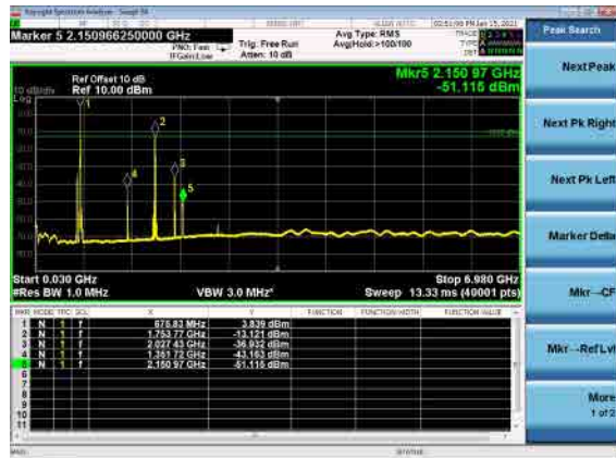
B66_N71(10M)_DFT-s-OFDM_BPSK_Mid_CH
