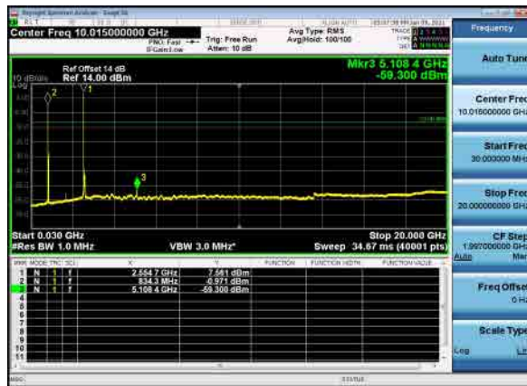
B26_N41(80M)_DFT-s-OFDM_QPSK_Mid_CH
