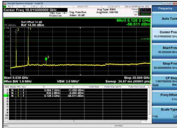
B26_N41(60M)_DFT-s-OFDM_QPSK_Mid_CH
