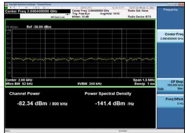
B26_N41(40M)_DFT-s-OFDM_QPSK_1RB_High_CH
