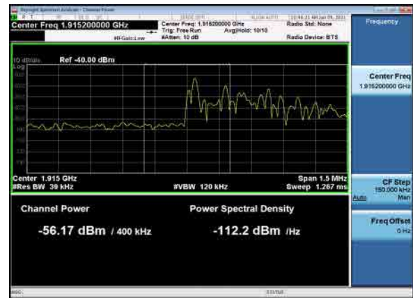
B12_N25(20M)_DFT-s-OFDM_BPSK_1RB_High_CH
