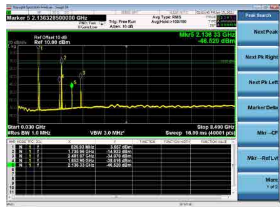
B66_N5(20M)_DFT-s-OFDM_QPSK_High_CH
