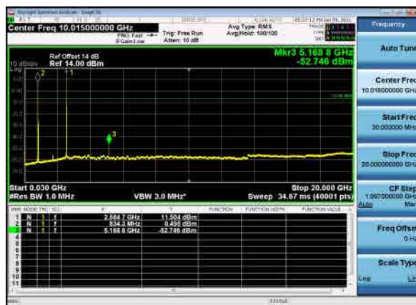
B26_N41(20M)_DFT-s-OFDM_BPSK_Mid_CH
