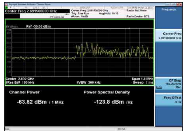
B26_N41(100M)_DFT-s-OFDM_QPSK_1RB_High_CH
