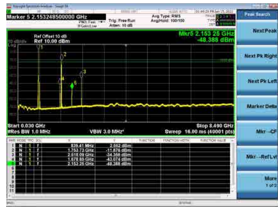
B66_N5(10M)_DFT-s-OFDM_QPSK_Mid_CH
