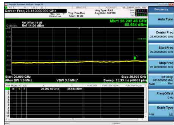
B26_N41(60M)_DFT-s-OFDM_QPSK_High_CH
