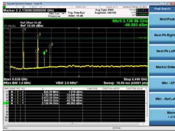
B66_N5(20M)_DFT-s-OFDM_BPSK_Low_CH
