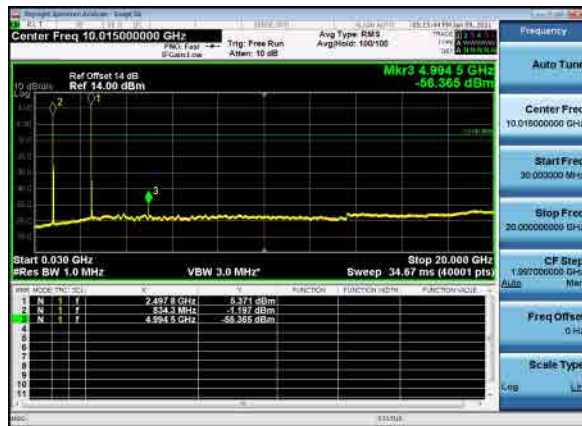
B26_N41(40M)_DFT-s-OFDM_BPSKe_Low_CH
