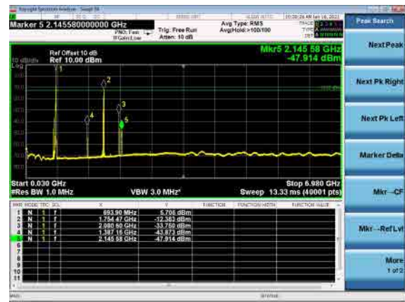
B66_N71(5M)_DFT-s-OFDM_QPSK_High_CH
