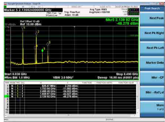
B66_N5(20M)_DFT-s-OFDM_QPSK_Mid_CH
