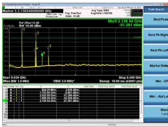
B66_N5(5M)_DFT-s-OFDM_BPSK_High_CH
