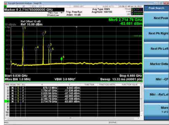
B66_N71(20M)_DFT-s-OFDM_QPSK_High_CH
