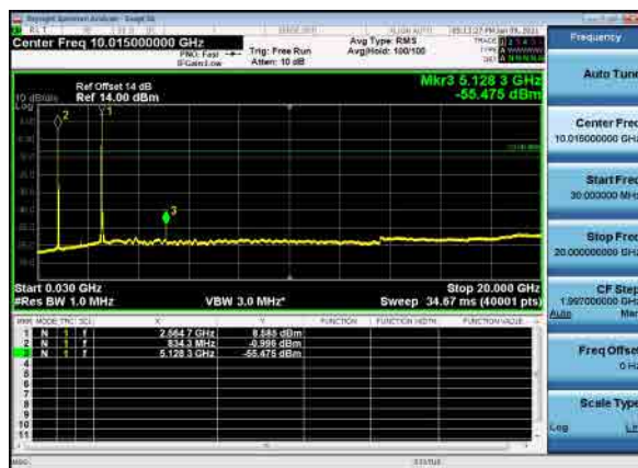
B26_N41(60M)_DFT-s-OFDM_BPSK_Mid_CH
