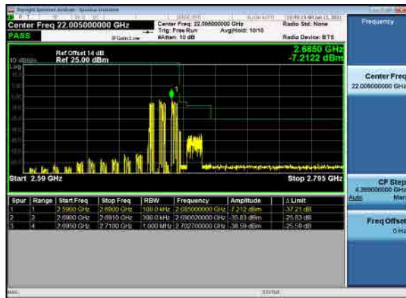
B26_N41(20M)_DFT-s-OFDM_QPSK_Full RB_High_CH
