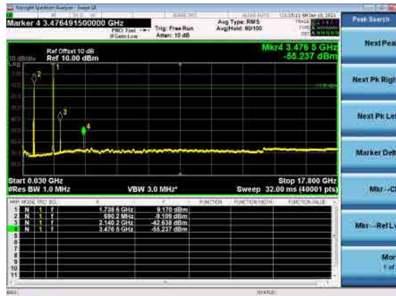
B71_N66(15M)_DFT-s-OFDM_BPSK_Mid_CH
