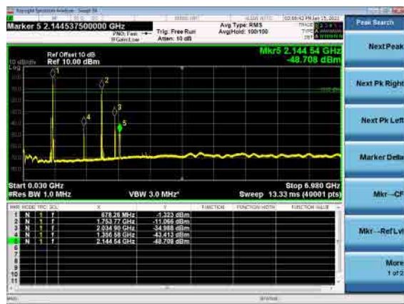
B66_N71(5M)_DFT-s-OFDM_BPSK_Mid_CH
