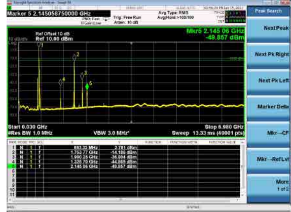
B66_N71(10M)_DFT-s-OFDM_QPSK_Low_CH
