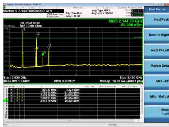
B66_N5(15M)_DFT-s-OFDM_BPSK_High_CH
