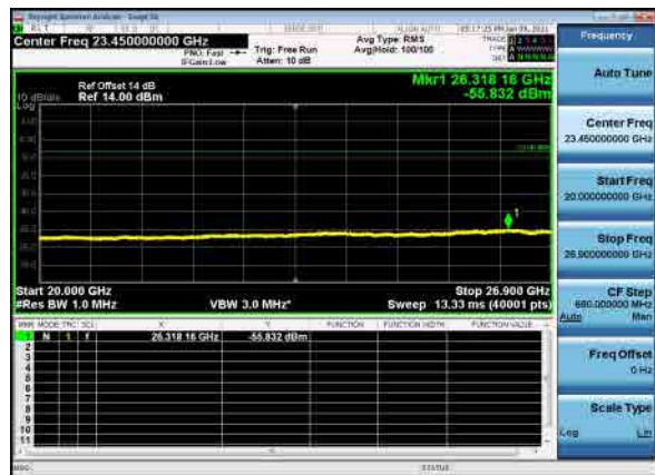
B26_N41(40M)_DFT-s-OFDM_QPSK_Low_CH
