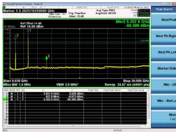
B26_N41(40M)_DFT-s-OFDM_BPSK_High_CH
