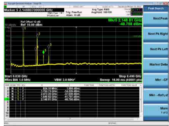
B66_N5(15M)_DFT-s-OFDM_QPSK_Low_CH
