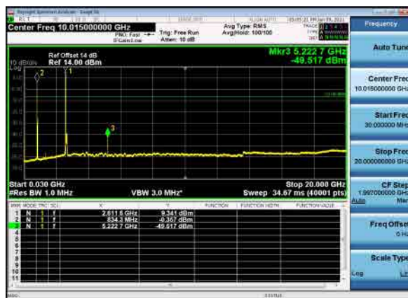
B26_N41(80M)_DFT-s-OFDM_QPSK_High_CH
