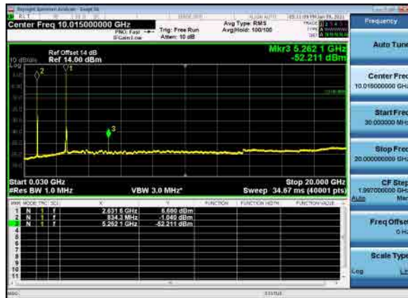
B26_N41(60M)_DFT-s-OFDM_BPSK_High_CH
