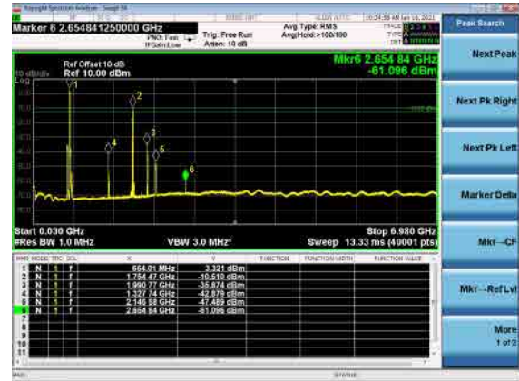
B66_N71(20M)_DFT-s-OFDM_QPSK_Low_CH
