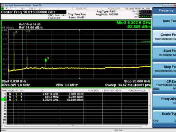
B26_N41(40M)_DFT-s-OFDM_QPSK_High_CH
