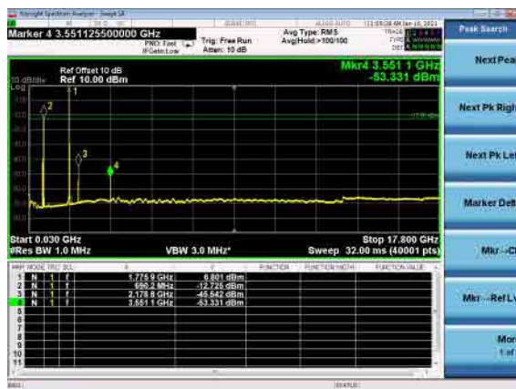
B71_N66(5M)_DFT-s-OFDM_BPSK_High_CH
