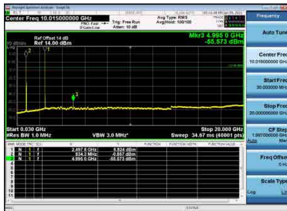
B26_N41(40M)_DFT-s-OFDM_QPSK_Low_CH
