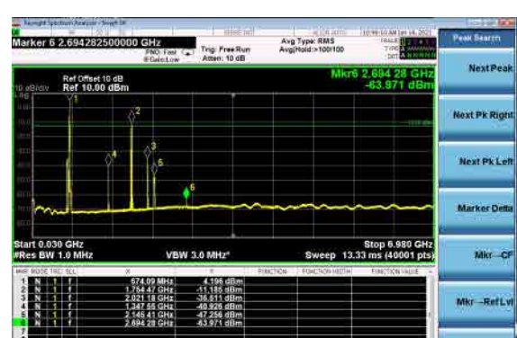
B66_N71(15M)_DFT-s-OFDM_QPSK_Mid_CH
