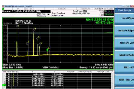
B66_N71(15M)_DFT-s-OFDM_BPSK_Mid_CH
