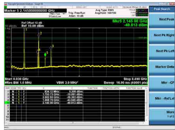
B66_N5(5M)_DFT-s-OFDM_QPSK_Mid_CH
