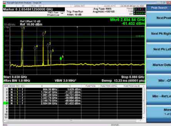
B66_N71(20M)_DFT-s-OFDM_BPSK_Low_CH
