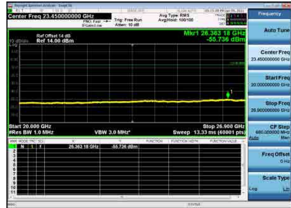
B26_N41(60M)_DFT-s-OFDM_QPSK_Mid_CH
