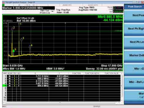
B71_N66(20M)_DFT-s-OFDM_BPSK_Low_CH
