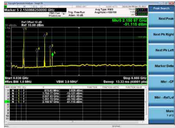
B66_N71(10M)_DFT-s-OFDM_QPSK_Mid_CH
