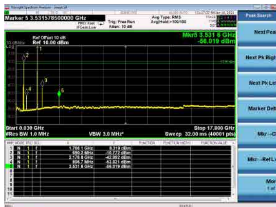
B71_N66(15M)_DFT-s-OFDM_BPSK_High_CH
