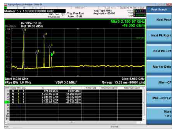
B66_N71(5M)_DFT-s-OFDM_QPSK_Mid_CH
