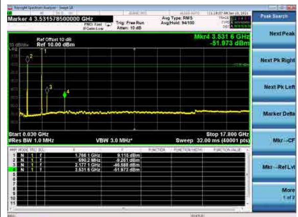
B71_N66(15M)_DFT-s-OFDM_QPSK_High_CH
