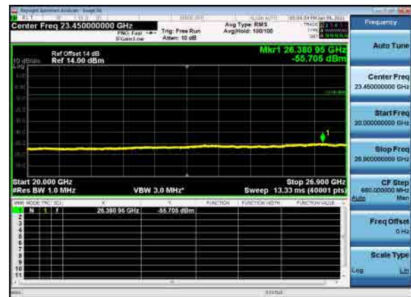
B26_N41(80M)_DFT-s-OFDM_BPSK_High_CH
