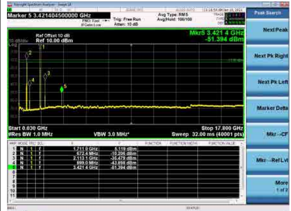
B71_N66(15M)_DFT-s-OFDM_QPSK_Low_CH
