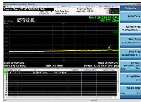
B26_N41(20M)_DFT-s-OFDM_BPSK_Mid_CH
