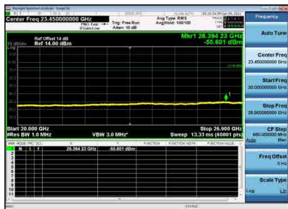
B26_N41(40M)_DFT-s-OFDM_BPSK_Mid_CH
