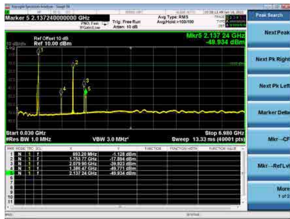
B66_N71(5M)_DFT-s-OFDM_BPSK_High_CH
