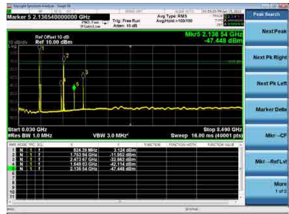
B66_N5(20M)_DFT-s-OFDM_QPSK_Low_CH
