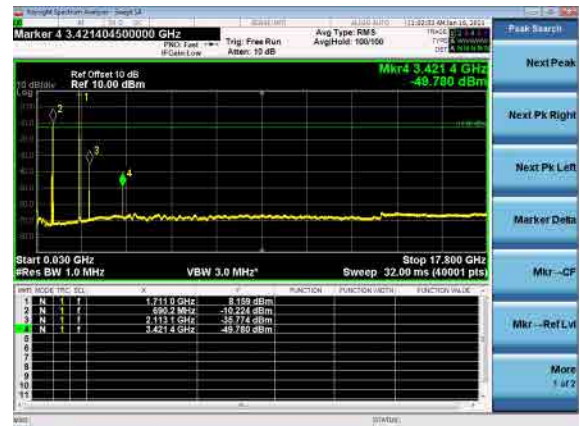
B71_N66(5M)_DFT-s-OFDM_QPSK_Low_CH
