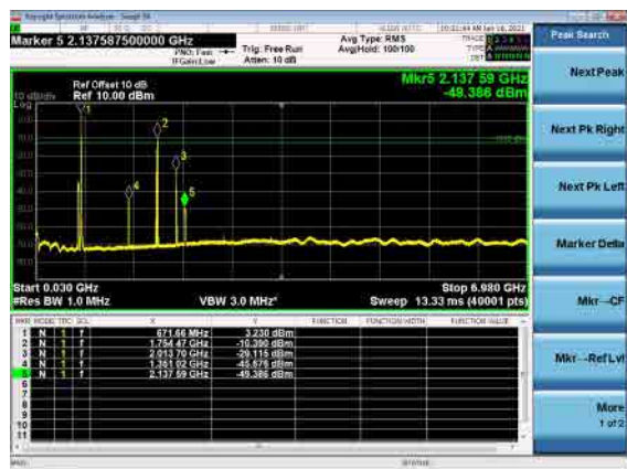
B66_N71(20M)_DFT-s-OFDM_BPSK_Mid_CH
