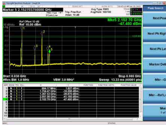
B66_N71(15M)_DFT-s-OFDM_BPSK_High_CH
