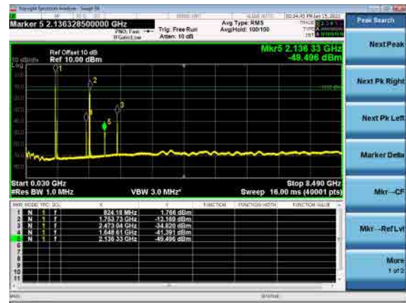
B66_N5(5M)_DFT-s-OFDM_QPSK_Low_CH
