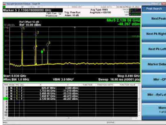
B66_N5(20M)_DFT-s-OFDM_BPSK_Mid_CH
