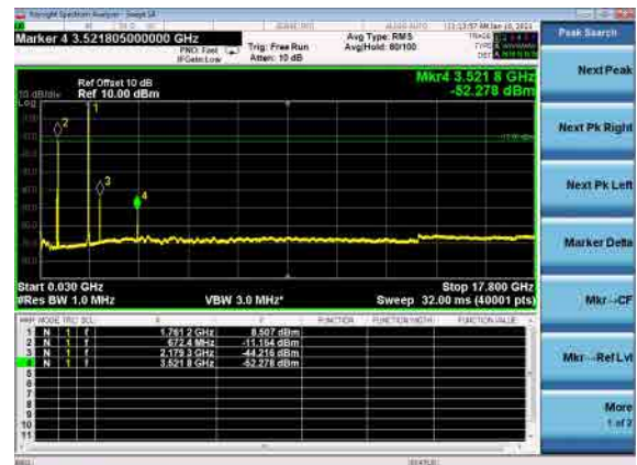
B71_N66(20M)_DFT-s-OFDM_QPSK_High_CH
