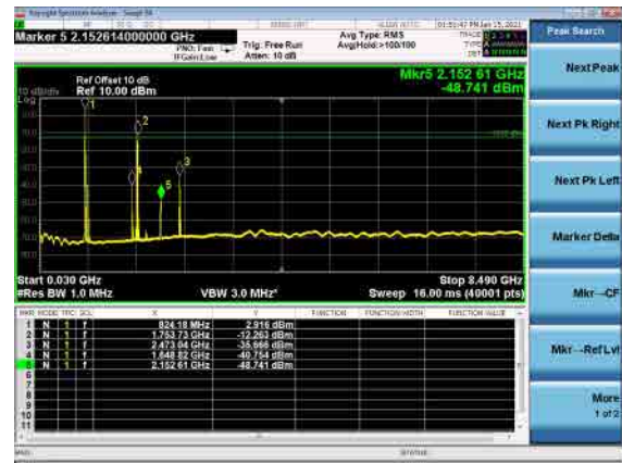
B66_N5(10M)_DFT-s-OFDM_QPSK_Low_CH
