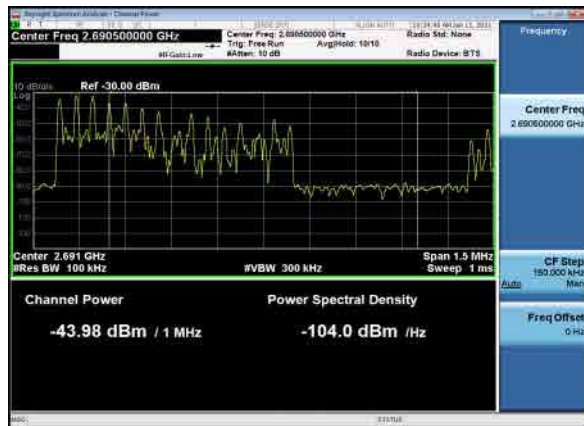
B26_N41(100M)_DFT-s-OFDM_QPSK_1RB_High_CH
