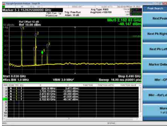
B66_N5(5M)_DFT-s-OFDM_BPSK_Low_CH
