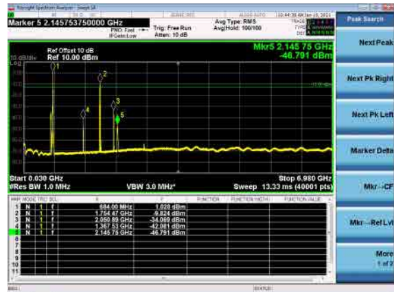
B66_N71(15M)_DFT-s-OFDM_QPSK_High_CH
