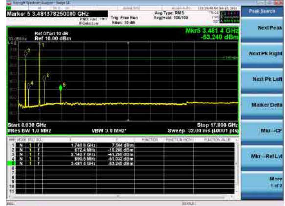
B71_N66(10M)_DFT-s-OFDM_QPSK_Mid_CH
