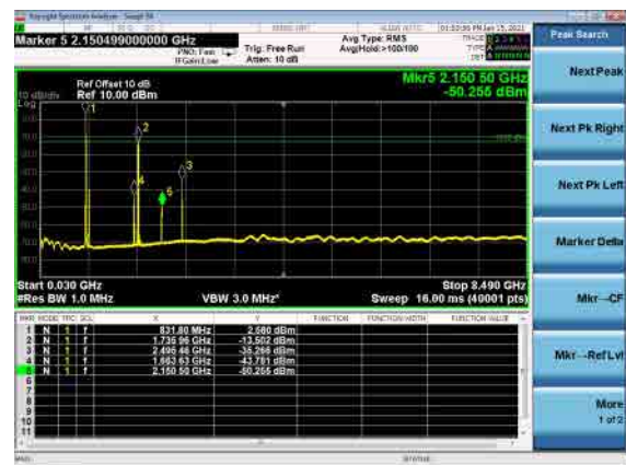
B66_N5(10M)_DFT-s-OFDM_QPSK_High_CH
