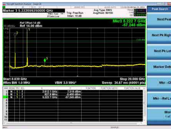
B26_N41(80M)_DFT-s-OFDM_BPSK_High_CH
