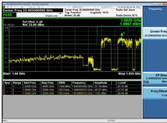
B12_N25(10M)_DFT-s-OFDM_BPSK_Full RB_Low_CH
