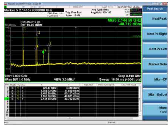
B66_N5(15M)_DFT-s-OFDM_QPSK_Mid_CH
