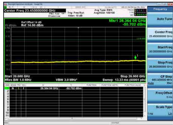
B26_N41(40M)_DFT-s-OFDM_QPSK_Mid_CH
