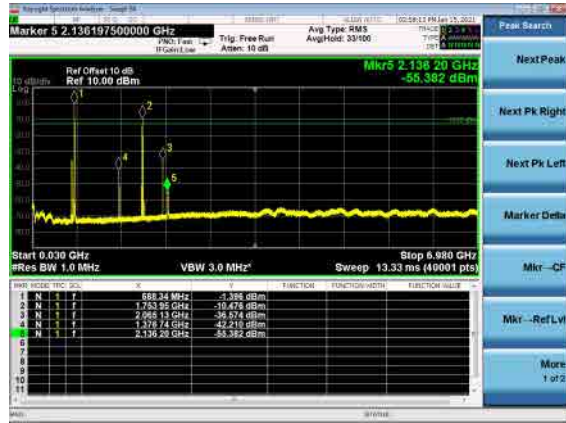
B66_N71(10M)_DFT-s-OFDM_BPSK_High_CH
