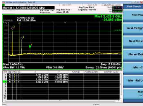
B71_N66(15M)_DFT-s-OFDM_BPSK_Low_CH
