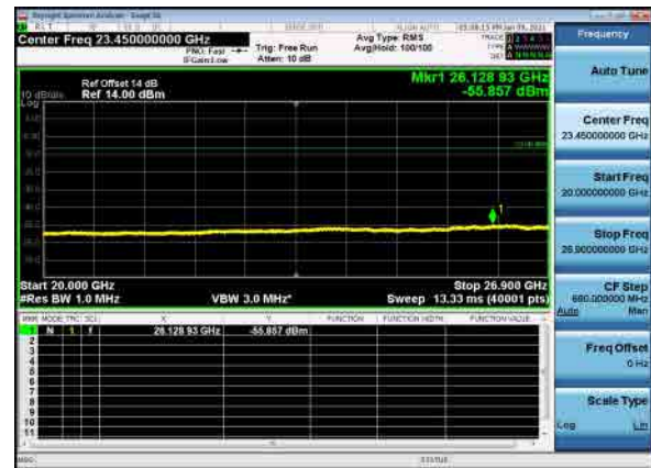
B26_N41(80M)_DFT-s-OFDM_QPSK_Mid_CH
