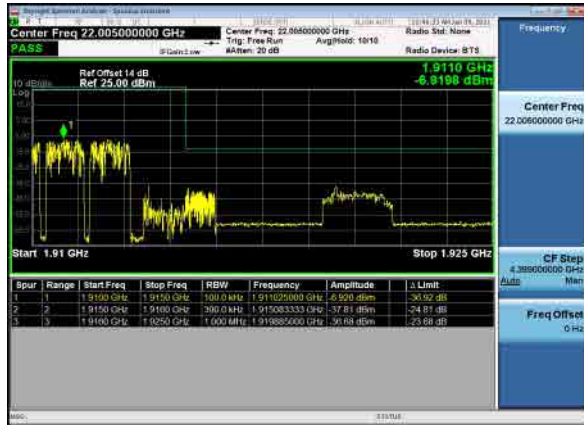
B12_N25(20M)_DFT-s-OFDM_QPSK_Full RB_High_CH
