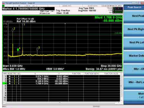
B26_N41(40M)_DFT-s-OFDM_QPSK_Mid_CH
