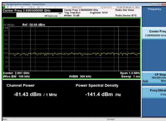
B26_N41(60M)_DFT-s-OFDM_BPSK_1RB_High_CH
