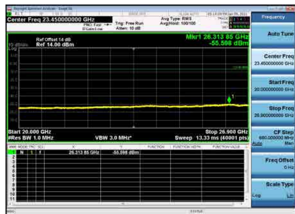
B26_N41(60M)_DFT-s-OFDM_BPSK_Mid_CH
