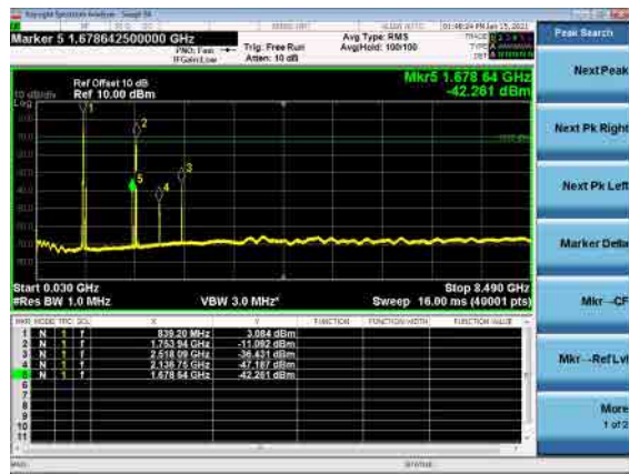
B66_N5(10M)_DFT-s-OFDM_BPSK_Mid_CH
