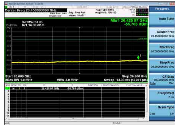
B26_N41(60M)_DFT-s-OFDM_BPSK_High_CH
