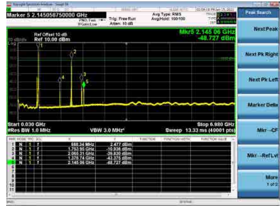
B66_N71(10M)_DFT-s-OFDM_QPSK_High_CH
