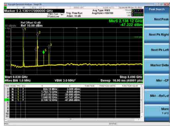
B66_N5(15M)_DFT-s-OFDM_QPSK_High_CH
