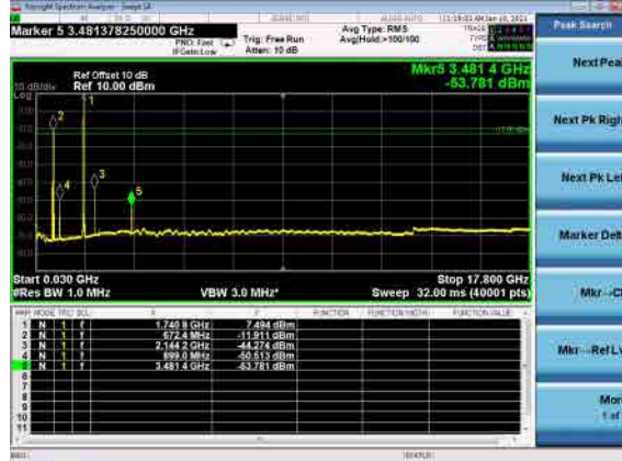
B71_N66(10M)_DFT-s-OFDM_BPSK_Mid_CH
