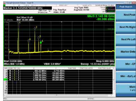
B66_N71(5M)_DFT-s-OFDM_QPSK_Low_CH
