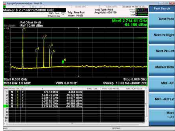
B66_N71(20M)_DFT-s-OFDM_BPSK_High_CH
