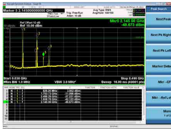
B66_N5(15M)_DFT-s-OFDM_BPSK_Mid_CH
