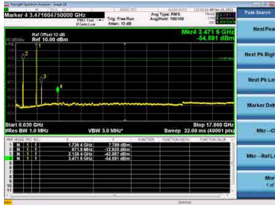
B71_N66(20M)_DFT-s-OFDM_BPSK_Mid_CH
