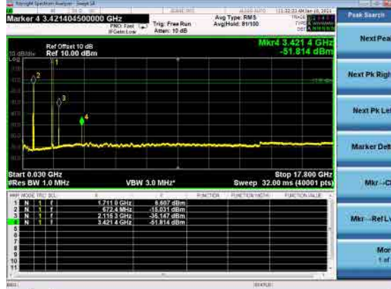
B71_N66(10M)_DFT-s-OFDM_BPSK_Low_CH
