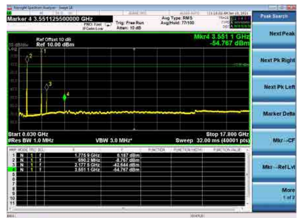
B71_N66(5M)_DFT-s-OFDM_QPSK_High_CH
