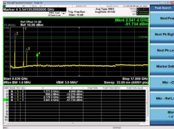
B71_N66(10M)_DFT-s-OFDM_BPSK_High_CH
