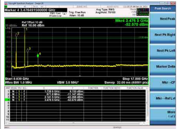
B71_N66(15M)_DFT-s-OFDM_QPSK_Mid_CH
