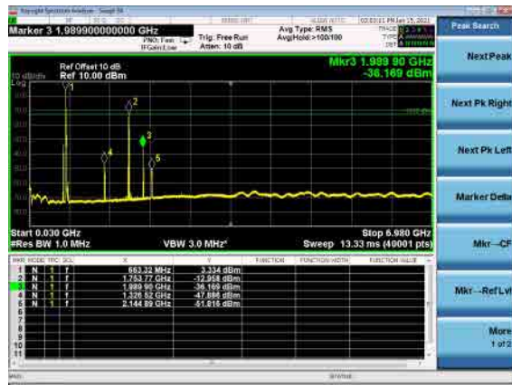
B66_N71(5M)_DFT-s-OFDM_BPSK_Low_CH
