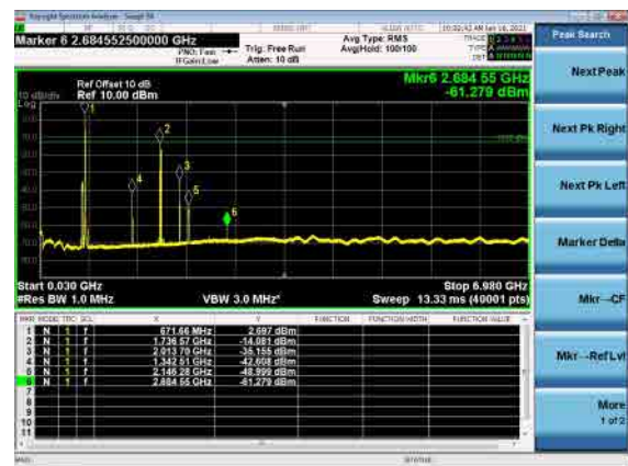
B66_N71(20M)_DFT-s-OFDM_QPSK_Mid_CH
