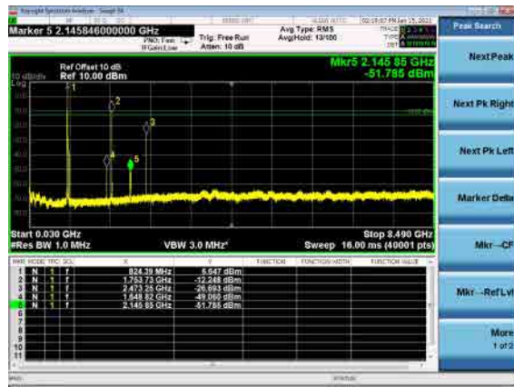
B66_N5(15M)_DFT-s-OFDM_BPSK_Low_CH
