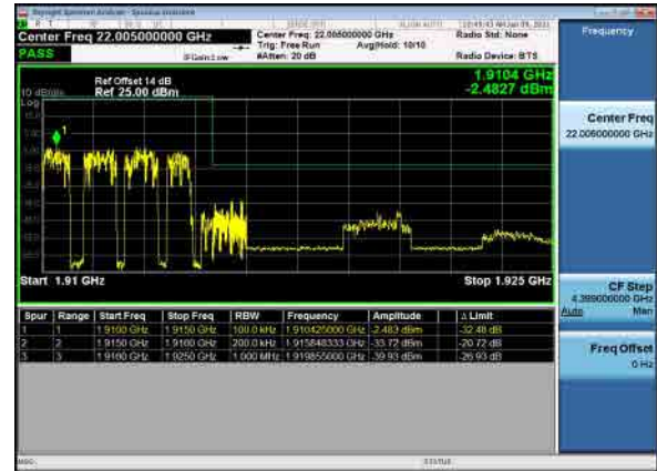
B12_N25(10M)_DFT-s-OFDM_QPSK_Full RB_High_CH
