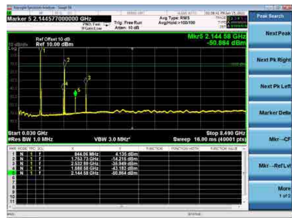
B66_N5(5M)_DFT-s-OFDM_QPSK_High_CH
