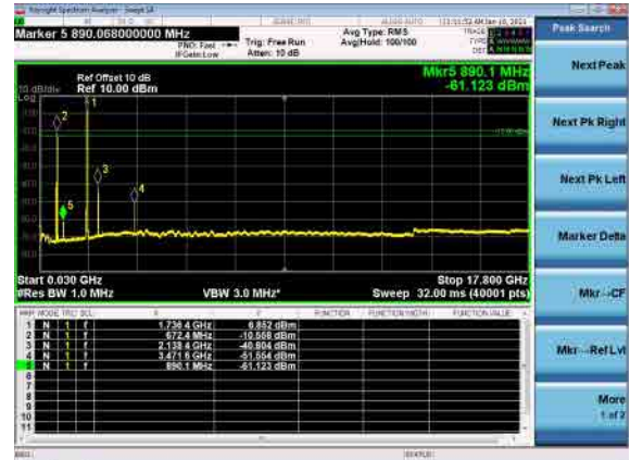
B71_N66(20M)_DFT-s-OFDM_QPSK_Mid_CH
