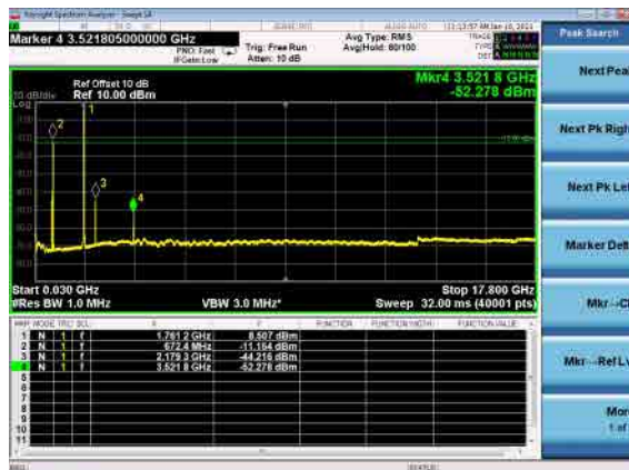
B71_N66(20M)_DFT-s-OFDM_BPSK_High_CH
