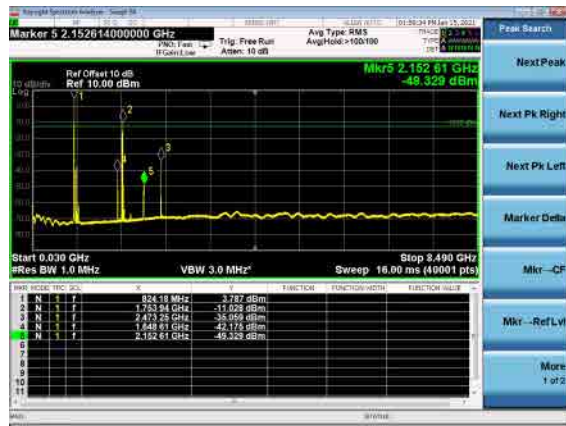
B66_N5(10M)_DFT-s-OFDM_BPSK_Low_CH
