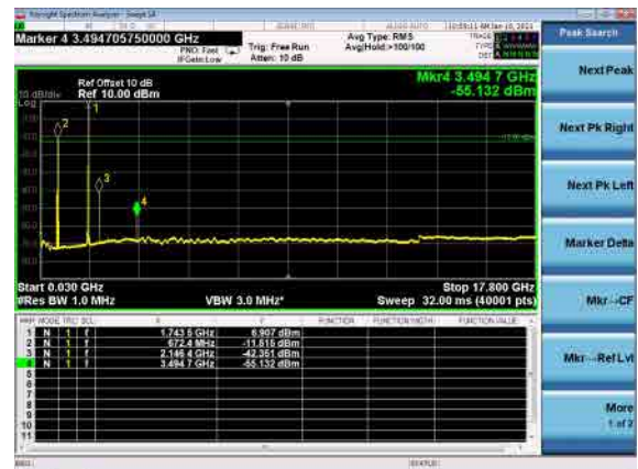
B71_N66(5M)_DFT-s-OFDM_QPSK_Mid_CH
