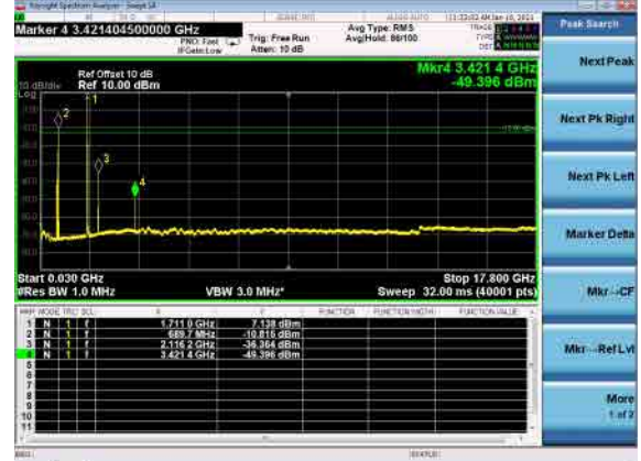
B71_N66(10M)_DFT-s-OFDM_QPSK_Low_CH
