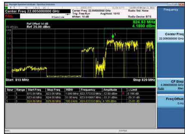
B66_N5(5M)_DFT-s-OFDM_BPSK_Full RB_Low_CH
