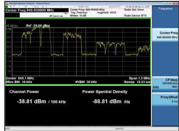
B66_N5(5M)_DFT-s-OFDM_BPSK_1RB_High_CH
