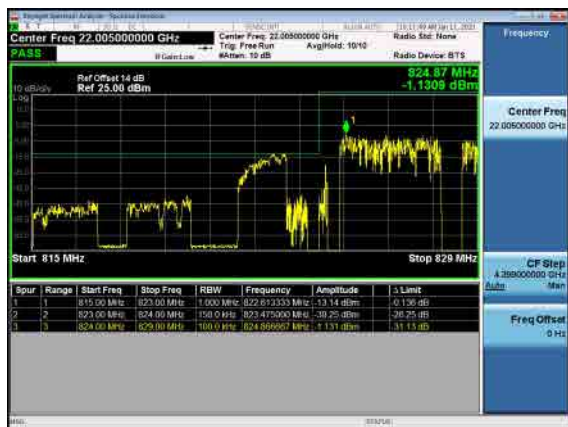
B66_N5(20M)_DFT-s-OFDM_BPSK_1RB_High_CH
