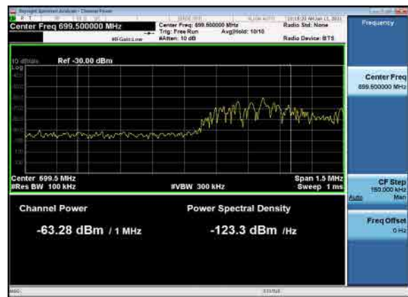
B66_N71(5M)_DFT-s-OFDM_QPSK_1RB_High_CH
