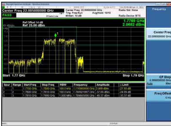
B71_N66(5M)_DFT-s-OFDM_BPSK_Full RB_High_CH
