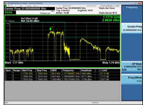
B71_N66(5M)_DFT-s-OFDM_QPSK_Full RB_High_CH
