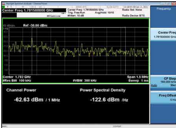
B71_N66(15M)_DFT-s-OFDM_QPSK_Full RB_High_CH
