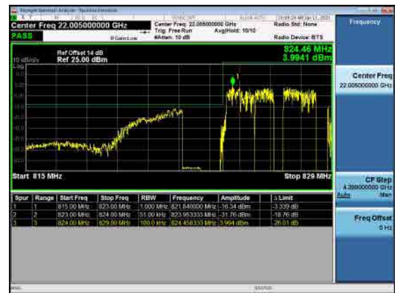
B66_N5(5M)_DFT-s-OFDM_QPSK_Full RB_Low_CH
