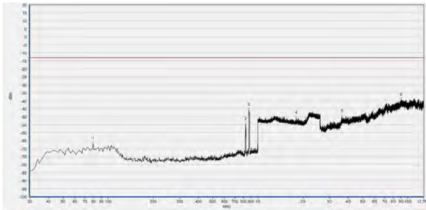
LTE Band 5, 10MHz BW, Low Channel, QPSK
