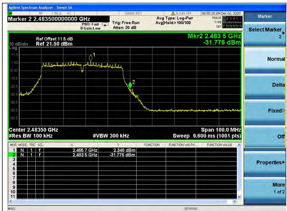
(Band Edge, Channel 11, 802.11n (HT40))
