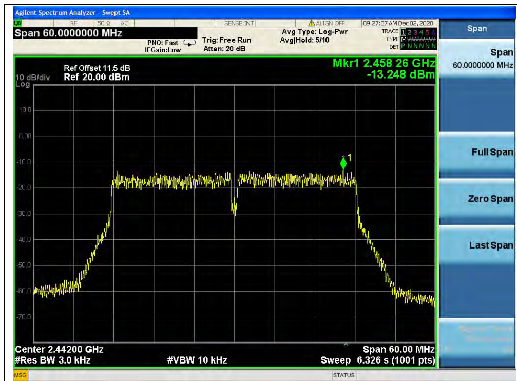
(Channel 7, 802.11n (HT40), ANT0)
