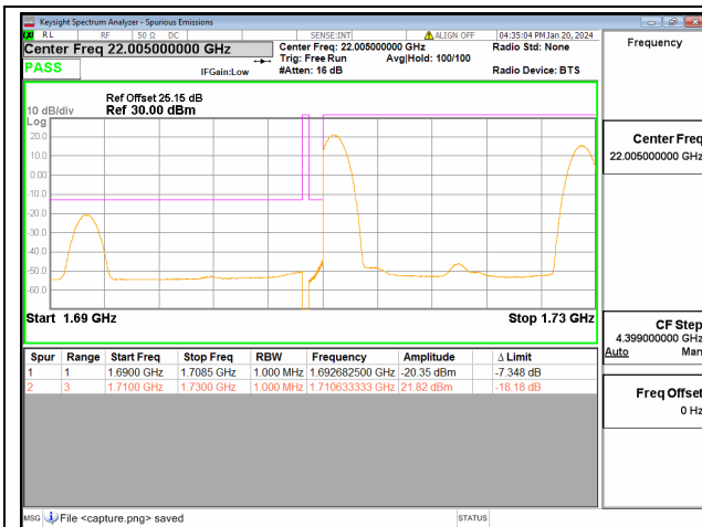
66B / 5+15MHz / Low CH / QPSK / 1#0-1#74
