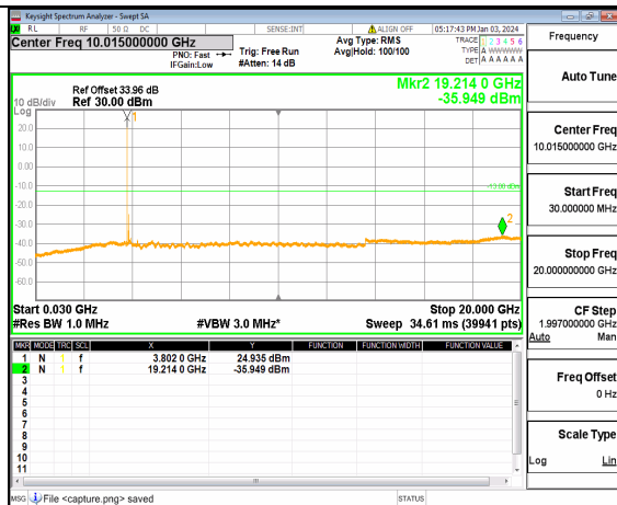
n77(3700-3980MHz) (30MHz-20GHz) 80M DFT-s-OFDM BPSK Inner 1RB Left Mid
