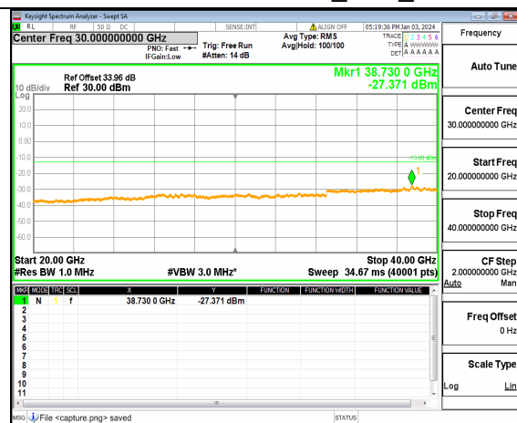
n77(3700-3980MHz) (20GHz-40GHz) 80M DFT-s-OFDM BPSK Inner 1RB Right Mid
