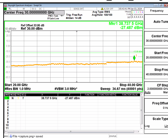
n77(3700-3980MHz) (20GHz-40GHz) 100M DFT-s-OFDM QPSK Inner 1RB Right High
