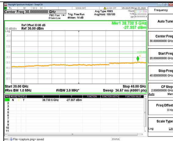
n77(3700-3980MHz) (20GHz-40GHz) 80M DFT-s-OFDM BPSK Inner 1RB Left Mid
