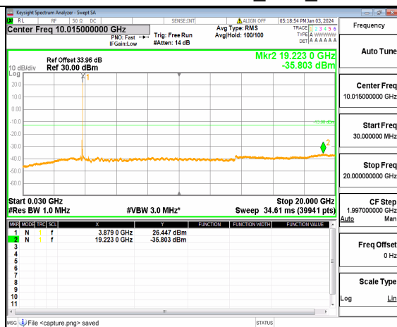
n77(3700-3980MHz) (30MHz-20GHz) 80M DFT-s-OFDM BPSK Inner 1RB Right Mid
