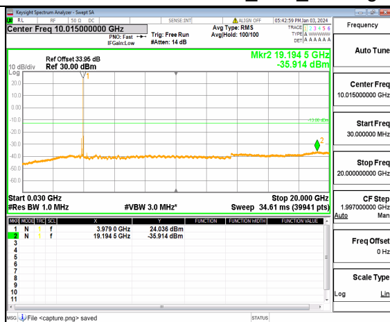
n77(3700-3980MHz) (30MHz-20GHz) 100M DFT-s-OFDM QPSK Inner 1RB Right High
