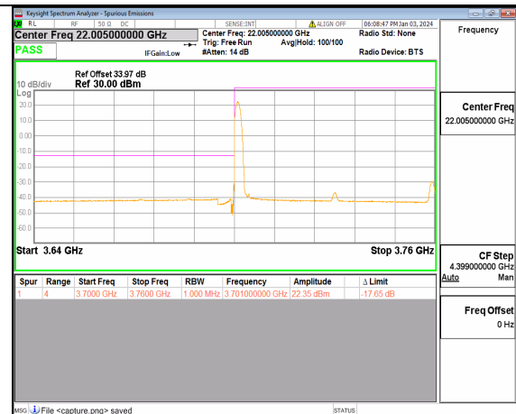
n77(3700-3980MHz) 60M DFT-s-OFDM QPSK Edge_1RB_Left Low
