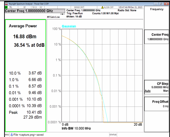
n2 10M CP-OFDM 256QAM Outer_Full Mid
