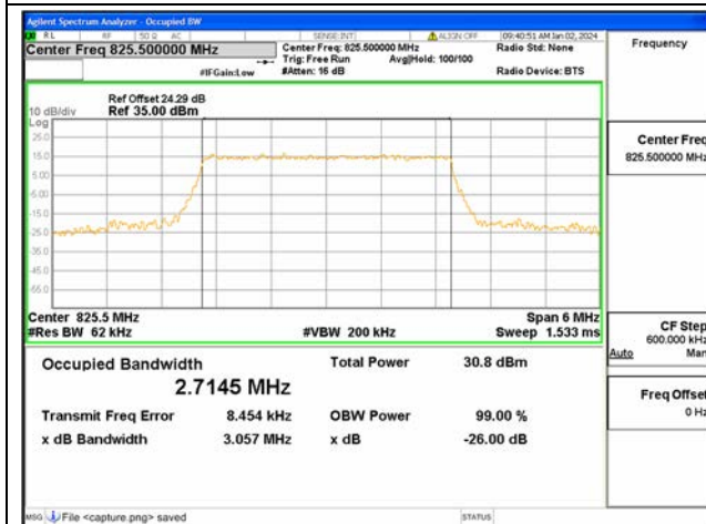
B5 / 3MHz / 16QAM/ Low CH
