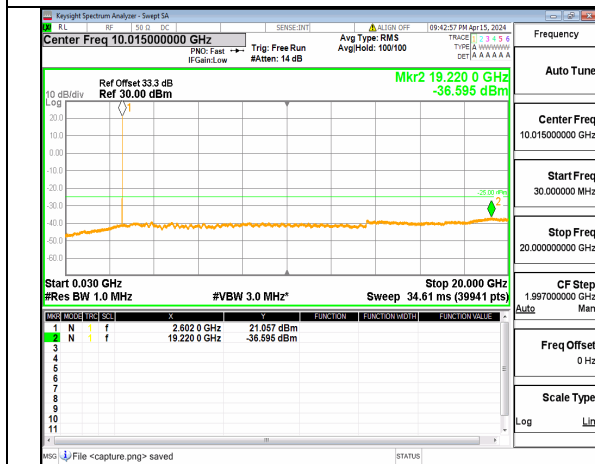
n41 (30MHz-20GHz) 20M DFT-s-OFDM BPSK Inner_1RB_Right Mid
