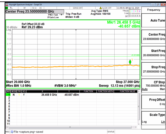
n41 (20GHz-27GHz) 20M DFT-s-OFDM BPSK Inner_1RB_Left Low
