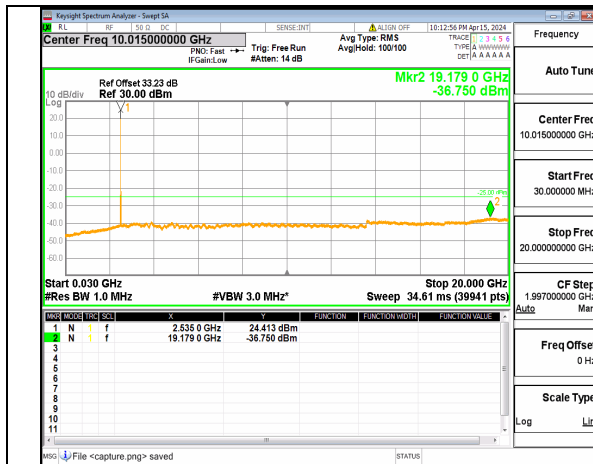
n41 (30MHz-20GHz) 40M DFT-s-OFDM QPSK Inner_1RB_Right Low
