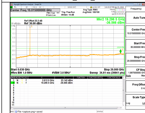
n41 (30MHz-20GHz) 40M DFT-s-OFDM BPSK Inner_1RB_Right Mid
