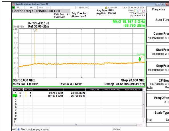
n41 (30MHz-20GHz) 40M DFT-s-OFDM BPSK Inner_1RB_Left Mid
