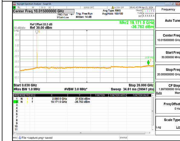
n41 (30MHz-20GHz) 20M DFT-s-OFDM BPSK Inner_1RB_Left Mid
