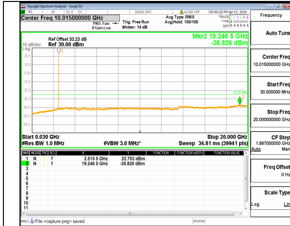
n41 (30MHz-20GHz) 20M DFT-s-OFDM QPSK Inner_1RB_Right Low
