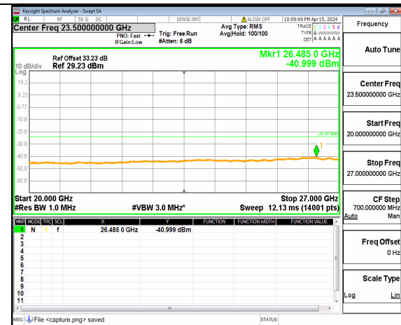
n41 (20GHz-27GHz) 40M DFT-s-OFDM BPSK Inner_1RB_Left Low
