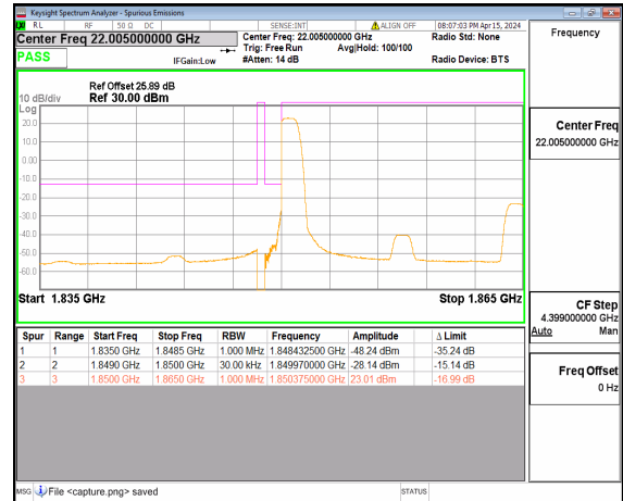
n25 15M DFT-s-OFDM BPSK Edge_1RB_Left Low
