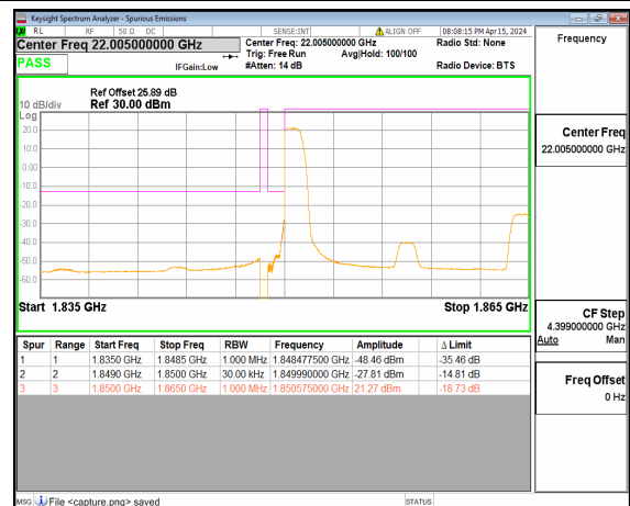
n25 15M DFT-s-OFDM 16QAM Edge_1RB_Left Low
