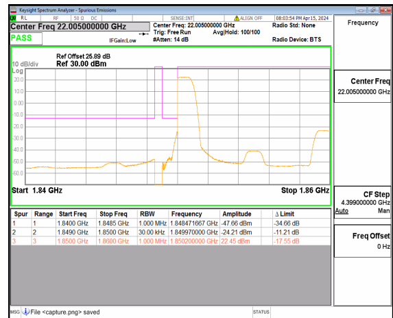
n25 10M DFT-s-OFDM BPSK Edge_1RB_Left Low
