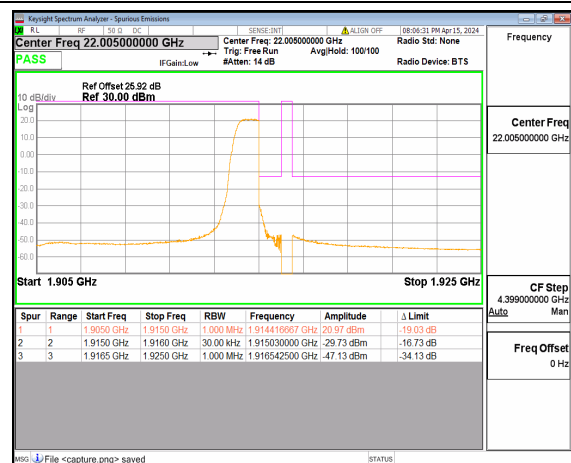
n25 10M DFT-s-OFDM 16QAM Edge_1RB_Right High
