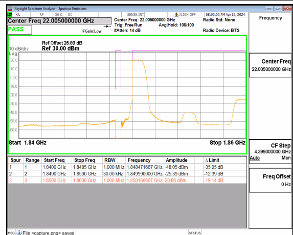
n25 10M DFT-s-OFDM 16QAM Edge_1RB_Left Low
