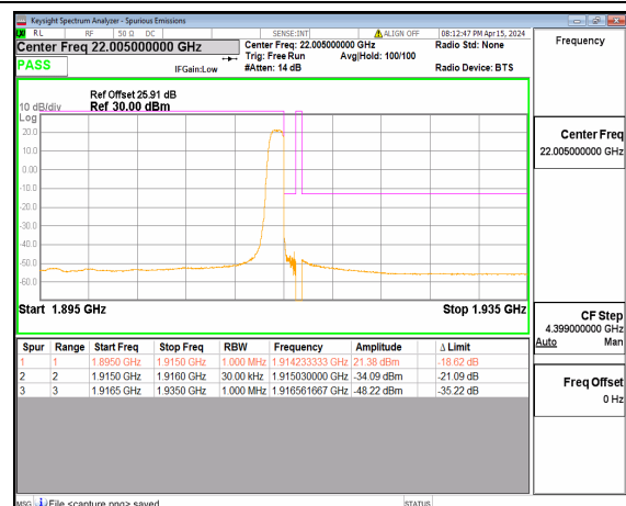
n25 20M DFT-s-OFDM 16QAM Edge_1RB_Right High
