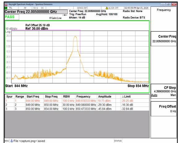
n26(824-849MHz) 5M DFT-s-OFDM BPSK Edge_1RB_Right High
