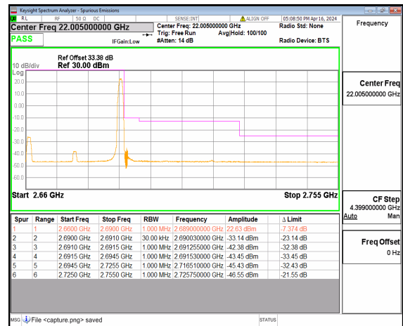
n41 30M DFT-s-OFDM BPSK Edge_1RB_Right High
