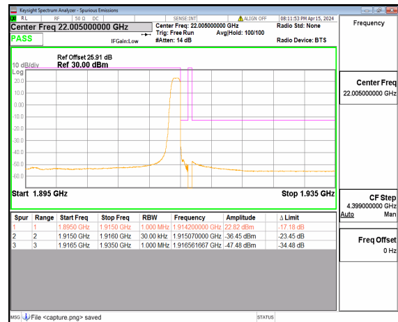
n25 20M DFT-s-OFDM BPSK Edge_1RB_Right High
