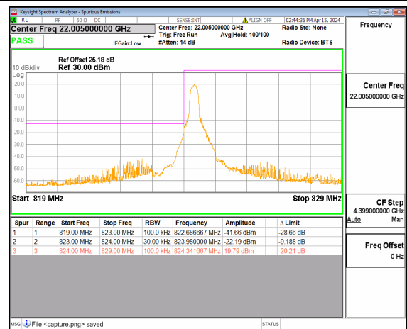
n26(824-849MHz) 5M DFT-s-OFDM BPSK Edge_1RB_Left Low
