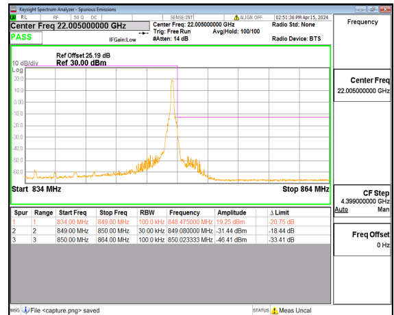
n26(824-849MHz) 15M DFT-s-OFDM QPSK Edge_1RB_Right High
