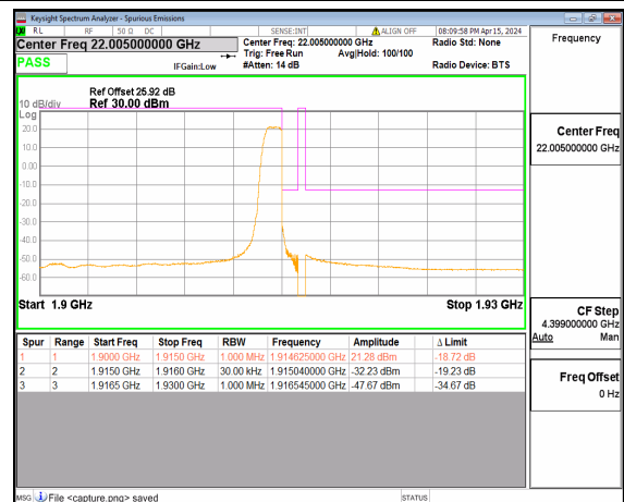
n25 15M DFT-s-OFDM 16QAM Edge_1RB_Right High
