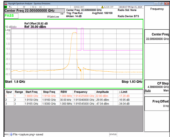
n25 15M DFT-s-OFDM BPSK Edge_1RB_Right High
