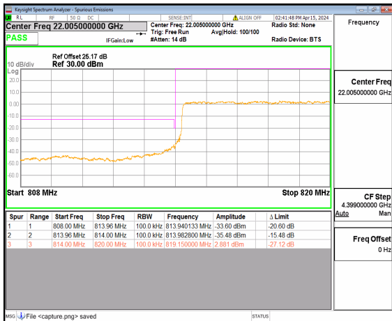
n26(814-824MHz) 10M DFT-s-OFDM BPSK Outer_Full Low
