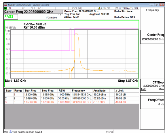
n25 20M DFT-s-OFDM 16QAM Edge_1RB_Left Low
