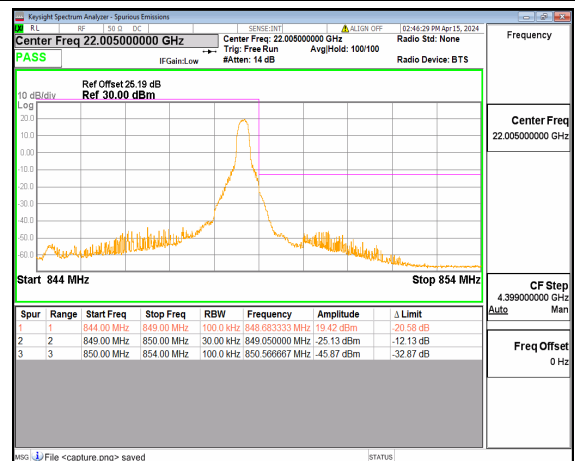
n26(824-849MHz) 5M DFT-s-OFDM QPSK Edge_1RB_Right High
