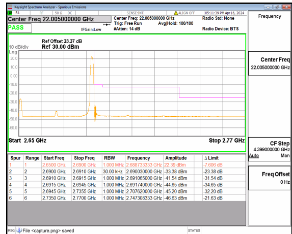
n41 40M DFT-s-OFDM BPSK Edge_1RB_Right High
