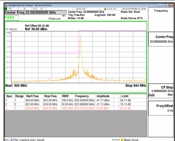
n26(824-849MHz) 20M DFT-s-OFDM BPSK Edge_1RB_Left Low
