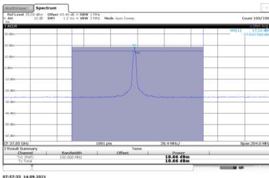
n260, Module1, 100MHz Bandwidth, 1 RB, LOW CHANNEL, QPSK
