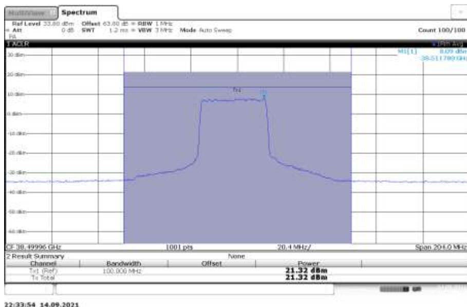
n260, Module1, 100MHz Bandwidth, 20RB, MID CHANNEL, QPSK
