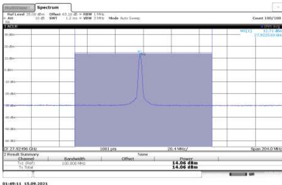
n261, Module1, 100MHz Bandwidth, 1RB, MID CHANNEL, QPSK
