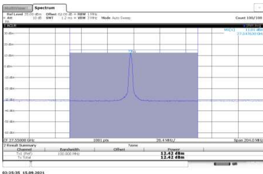
n261, Module1, 100MHz Bandwidth, 1 RB, LOW CHANNEL, QPSK
