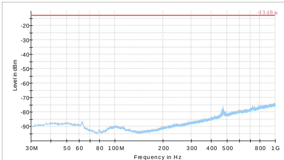
30MHz-1GHz
