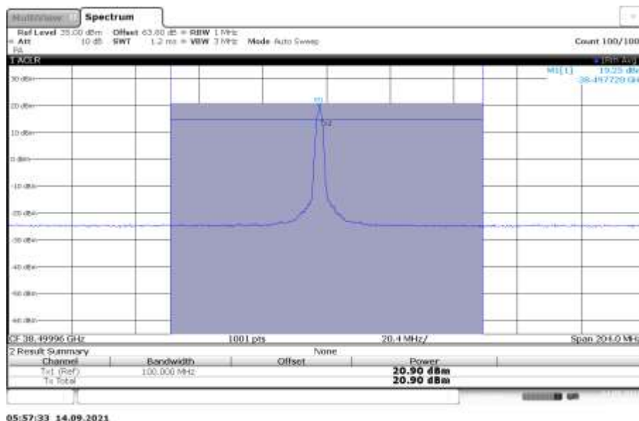
n260, Module1, 100MHz Bandwidth, 1RB, MID CHANNEL, QPSK
