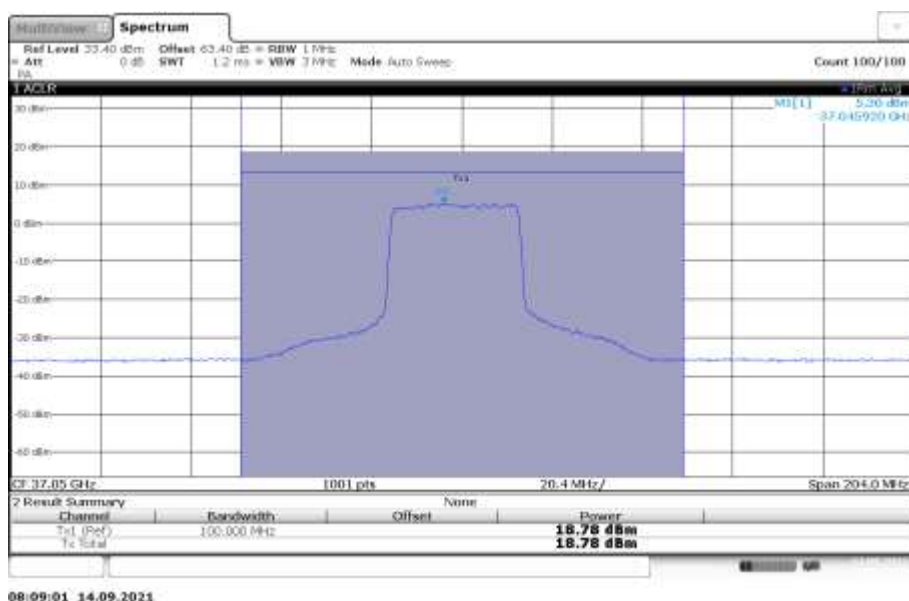
n260, Module1, 100MHz Bandwidth, 20 RB, LOW CHANNEL, QPSK
