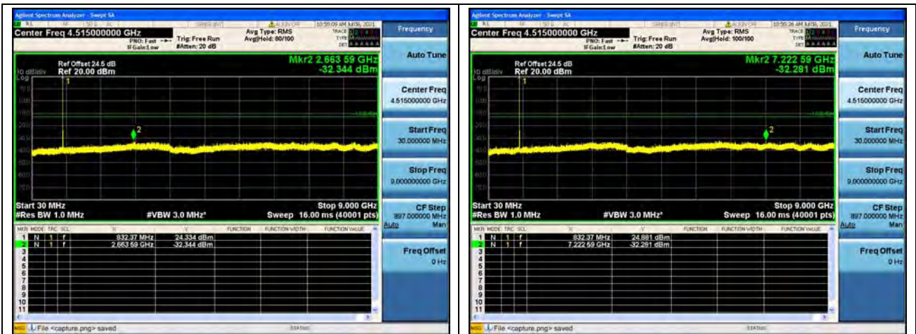
Band5 / 10MHz / Mid CH / 64QAM
