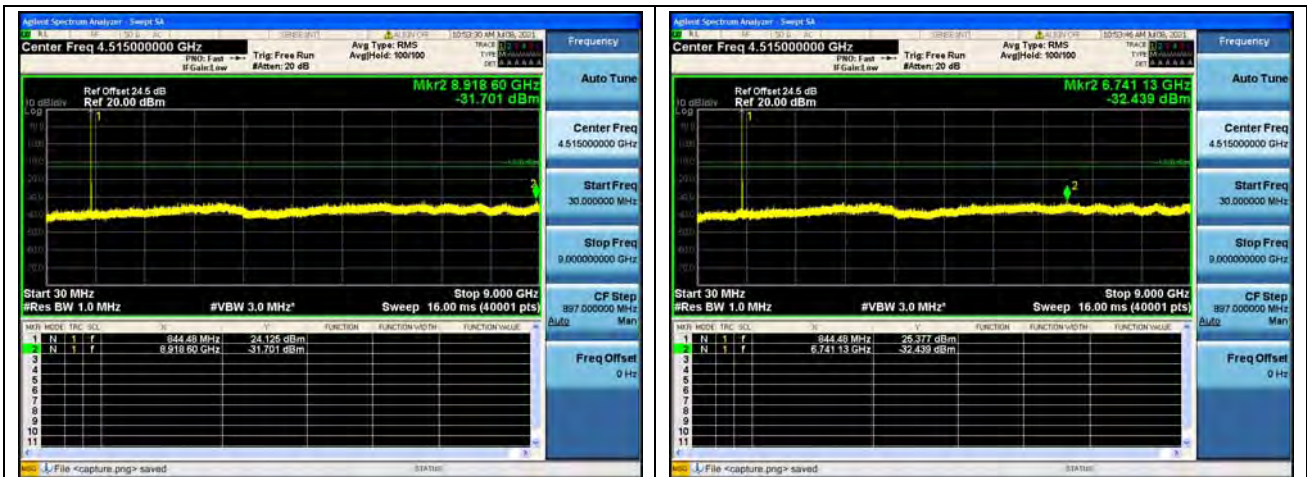
Band5 / 5MHz / High CH / 64QAM
