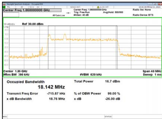
B13_N2(20M)_DFT-s-OFDM_16 QAM_Outer_Full_Low_CH
