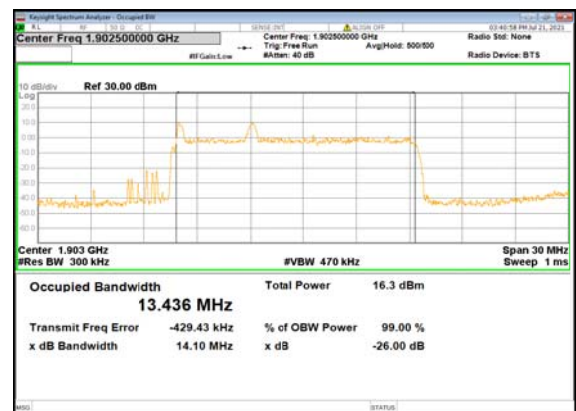
B13_N2(15M)_DFT-s-OFDM_QPSK_Outer _Full_High_CH
