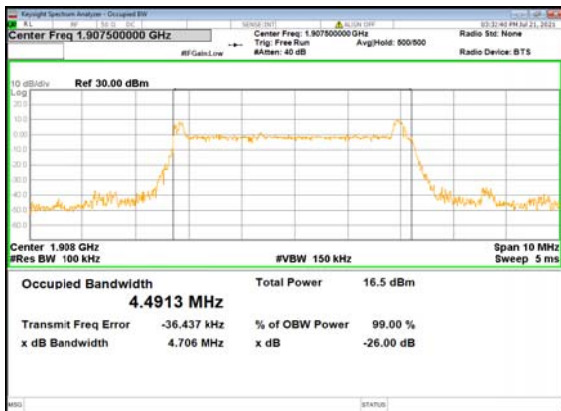
B13_N2(5M)_DFT-s-OFDM_16 QAM_Outer_Full_High_CH
