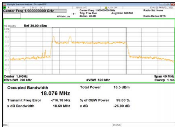
B13_N2(20M)_DFT-s-OFDM_16 QAM_Outer_Full_High_CH
