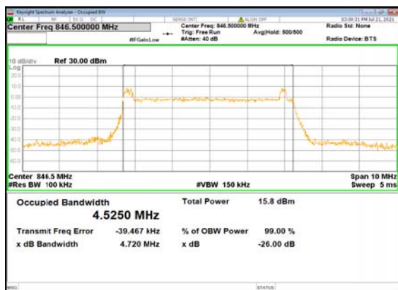
B2_N5(5M)_DFT-s-OFDM_PI_2-BPSK_Outer_Full _High_CH
