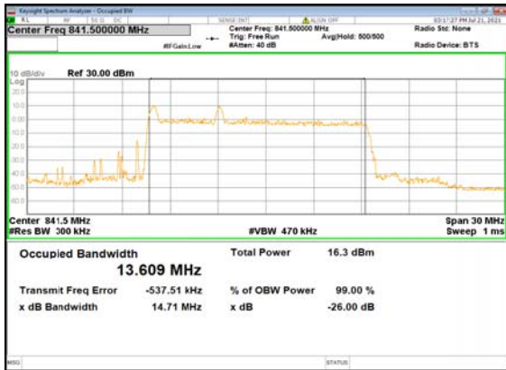
B2_N5(15M)_DFT-s-OFDM_16 QAM_Outer_Full_High_CH
