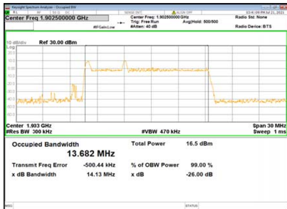
B13_N2(15M)_DFT-s-OFDM_16 QAM_Outer_Full_High_CH
