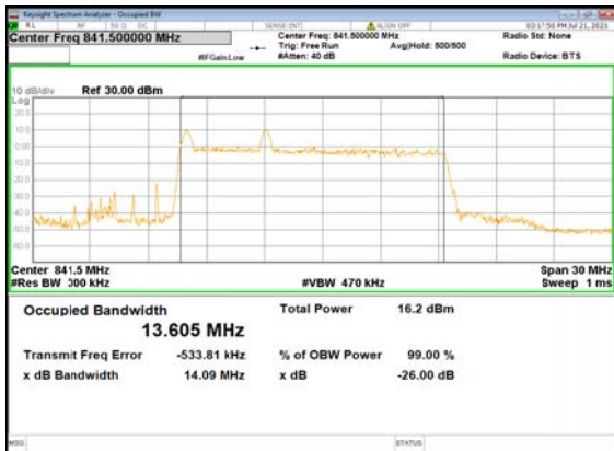
B2_N5(15M)_DFT-s-OFDM_256 QAM_Outer_Full_High_CH
