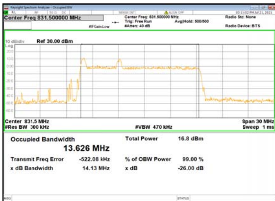
B2_N5(15M)_DFT-s-OFDM_256 QAM_Outer_Full_Low_CH
