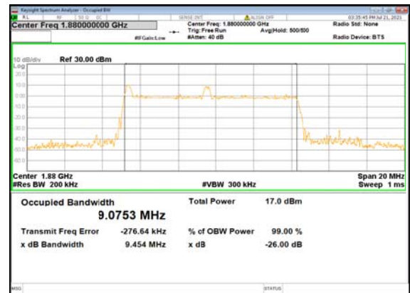
B13_N2(10M)_DFT-s-OFDM_64 QAM_Outer_Full_Mid_CH
