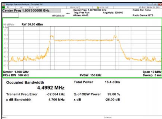
B13_N2(5M)_DFT-s-OFDM_256 QAM_Outer_Full_High_CH
