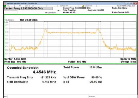
B13_N2(5M)_DFT-s-OFDM_64 QAM_Outer_Full_Low_CH
