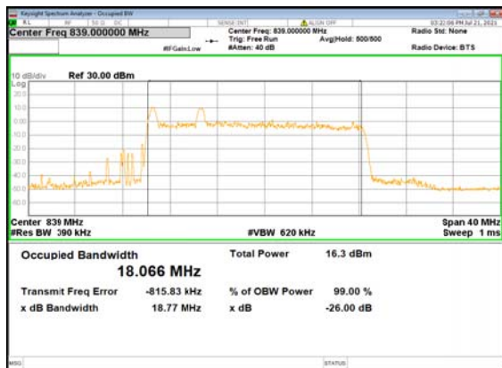
B2_N5(20M)_DFT-s-OFDM_256 QAM_Outer_Full_High_CH
