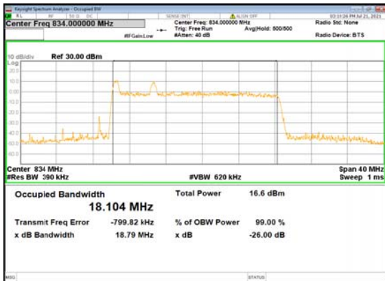
B2_N5(20M)_DFT-s-OFDM_PI_2-BPSK_Outer_Ful l_Low_CH
