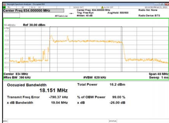
B2_N5(20M)_DFT-s-OFDM_16 QAM_Outer_Full_Low_CH
