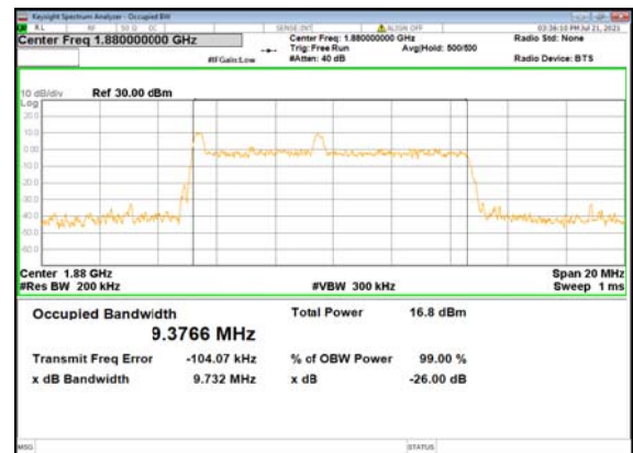
B13_N2(10M)_CP-OFDM_QPSK_Outer_F ull_Mid_CH
