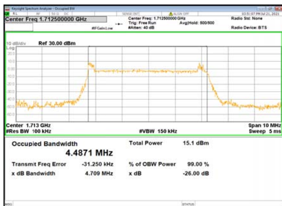
B13_N66(5M)_DFT-s-OFDM_PI_2-BPSK_Outer_F ull_Low_CH
