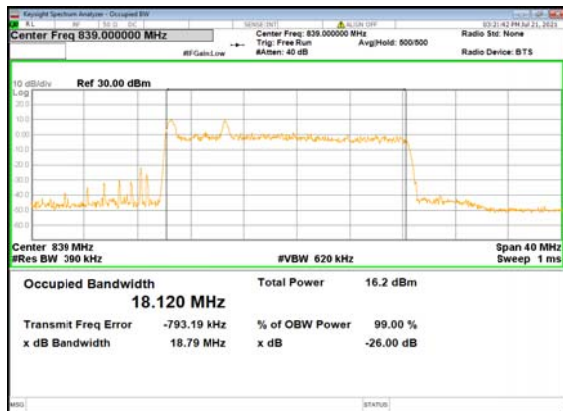
B2_N5(20M)_DFT-s-OFDM_16 QAM_Outer_Full_High_CH
