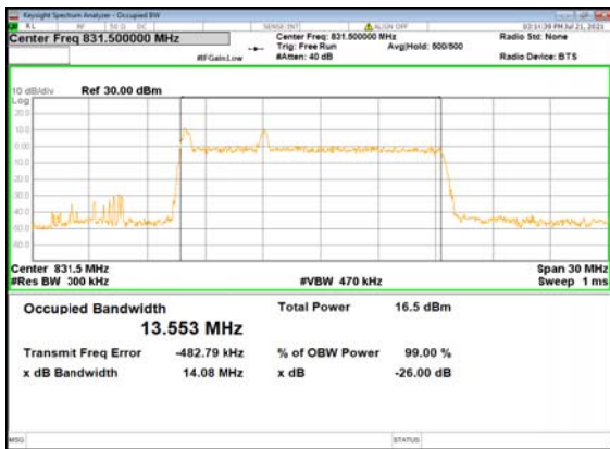
B2_N5(15M)_DFT-s-OFDM_16 QAM_Outer_Full_Low_CH
