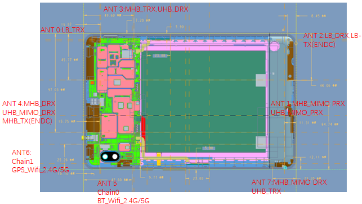
Fig.11.1 EUT Antenna Locations
