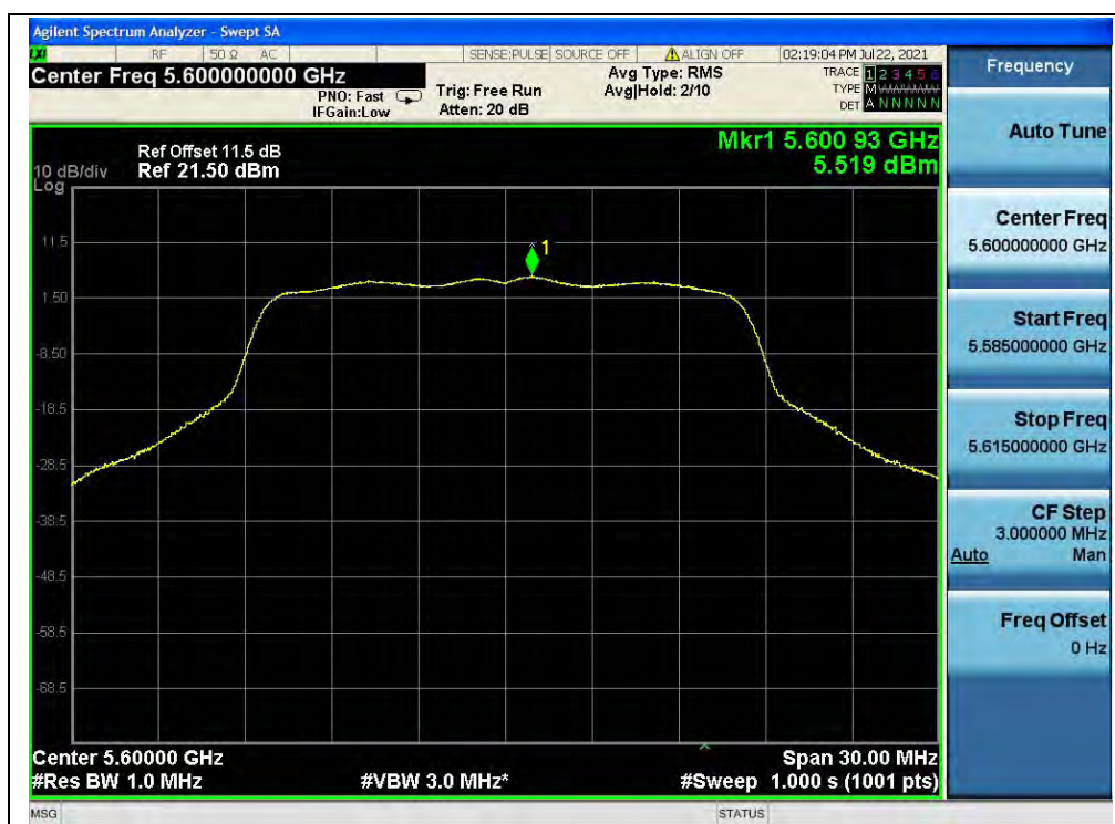
(Channel 120, 5600MHz, 802.11a, ANT1)
