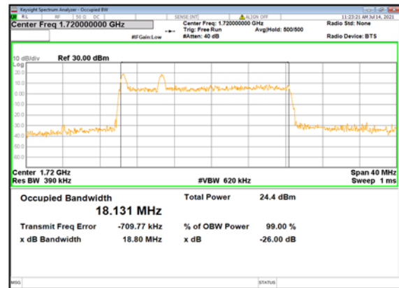
n66(20M)_DFT-s-OFDM_ 64QAM_Outer_Full_Low_CH
