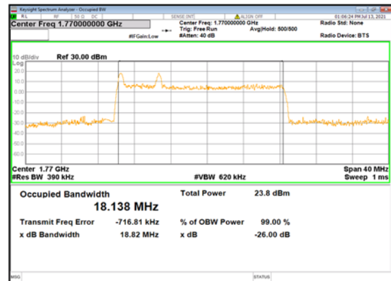
n66(20M)_CP-OFDM_ QPSK_Outer_Full_High_CH
