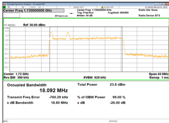
n66(20M)_DFT-s-OFDM_ 256QAM_Outer_Full_Low_CH
