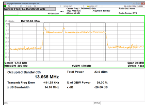
n66(15M)_DFT-s-OFDM_ 64QAM_Outer_Full_Mid_CH
