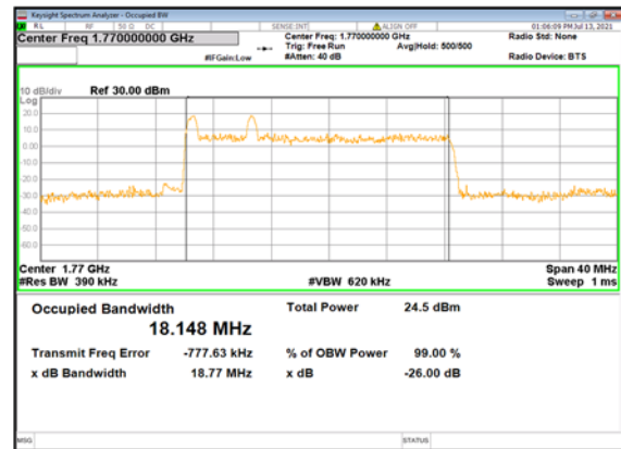
n66(20M)_DFT-s-OFDM_ 64QAM_Outer_Full_High_CH
