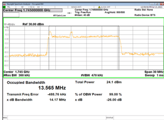
n66(15M)_DFT-s-OFDM_ 16QAM_Outer_Full_Mid_CH
