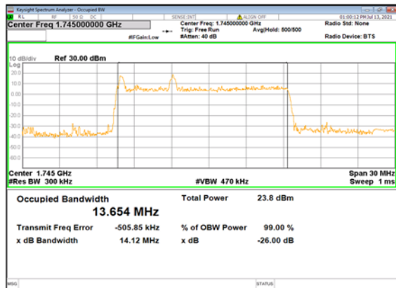
n66(15M)_DFT-s-OFDM_ 256QAM_Outer_Full_Mid_CH
