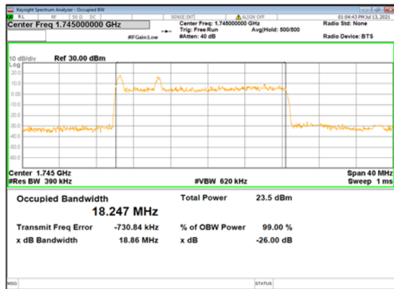
n66(20M)_DFT-s-OFDM_ 256QAM_Outer_Full_Mid_CH
