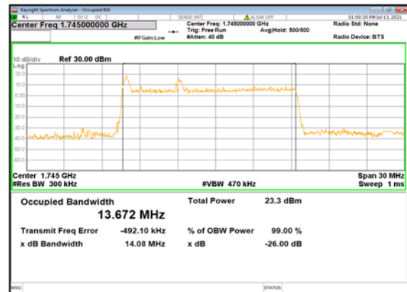
n66(15M)_CP-OFDM_ QPSK_Outer_Full_Mid_CH
