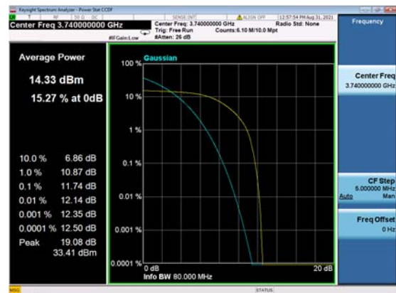
DC_13A_n77(80M)_DFT-s-OFDM_ QPSK_Outer_Full_Low_CH
