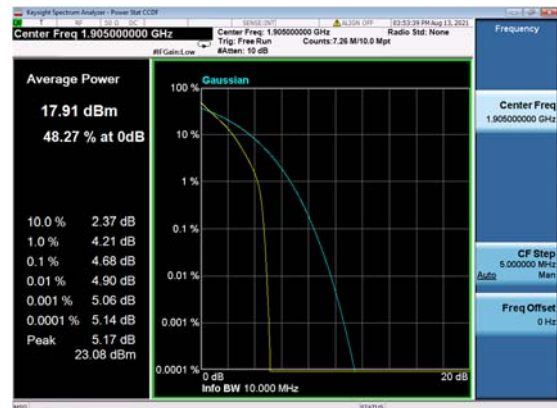
n2(10M)_DFT-s-OFDM_ QPSK_Outer_Full_High_CH
