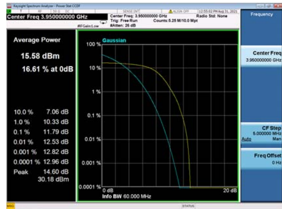
DC_13A_n77(60M)_DFT-s-OFDM_ QPSK_Outer_Full_High_CH
