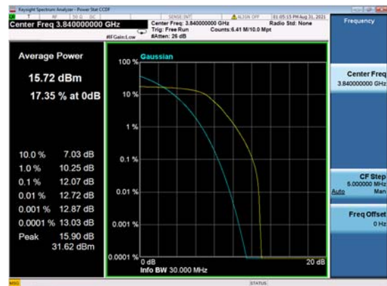
DC_13A_n77(30M)_DFT-s-OFDM_ QPSK_Outer_Full_Mid_CH
