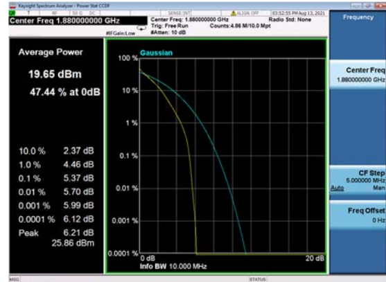
n2(10M)_DFT-s-OFDM_ QPSK_Outer_Full_Mid_CH
