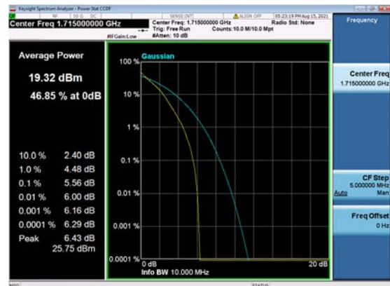
n66(10M)_DFT-s-OFDM_ QPSK_Outer_Full_Low_CH
