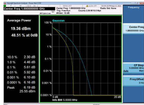
n2(5M)_DFT-s-OFDM_ QPSK_Outer_Full_Mid_CH
