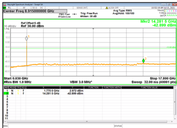
n66(5M)_DFT-s-OFDM_BPSK_Edge_1RB_ Left_High_CH
