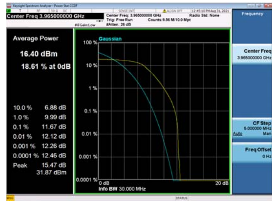
DC_13A_n77(30M)_DFT-s-OFDM_ QPSK_Outer_Full_High_CH
