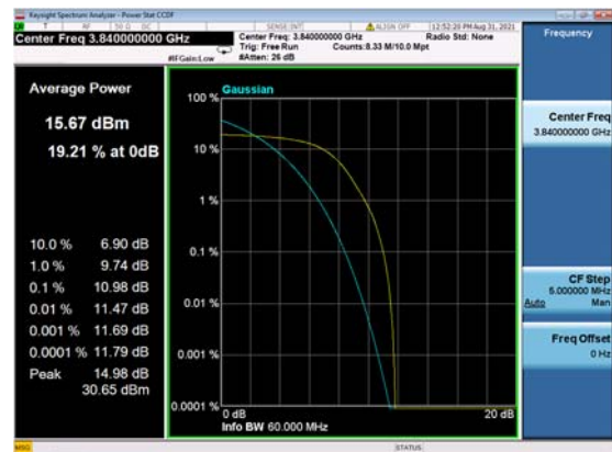
DC_13A_n77(60M)_DFT-s-OFDM_ QPSK_Outer_Full_Mid_CH
