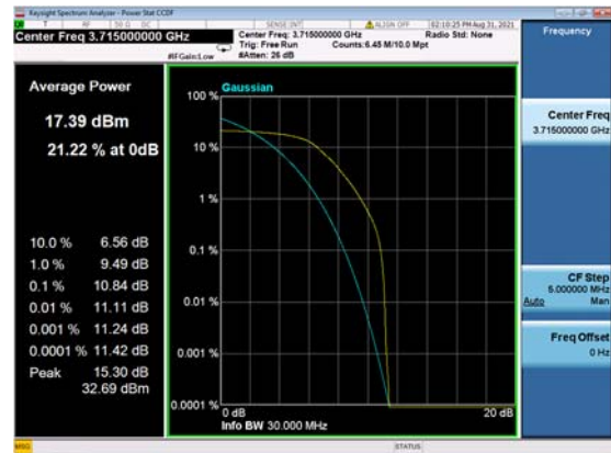
DC_13A_n77(30M)_DFT-s-OFDM_ QPSK_Outer_Full_Low_CH
