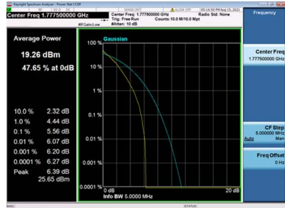
n66(5M)_DFT-s-OFDM_ QPSK_Outer_Full_High_CH
