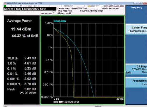
n2(20M)_DFT-s-OFDM_ QPSK_Outer_Full_Low_CH
