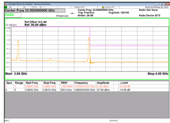
DC_13A_n77(100M)_DFT-s-OFDM_ QPSK_Edge_1RB_Right_High_CH
