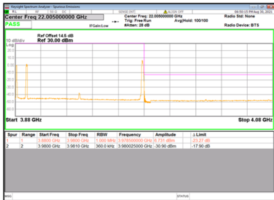
DC_13A_n77(100M)_DFT-s-OFDM_ BPSK_Edge_1RB_Right_High_CH
