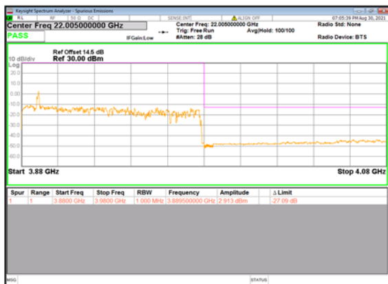
DC_13A_n77(100M)_DFT-s-OFDM_ BPSK_Outer_Full_High_CH
