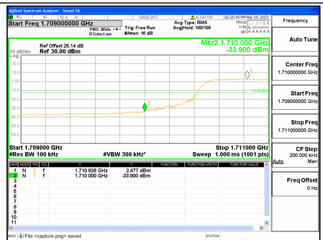
Band4 / 10MHz / Low CH / QPSK / FULL RB
