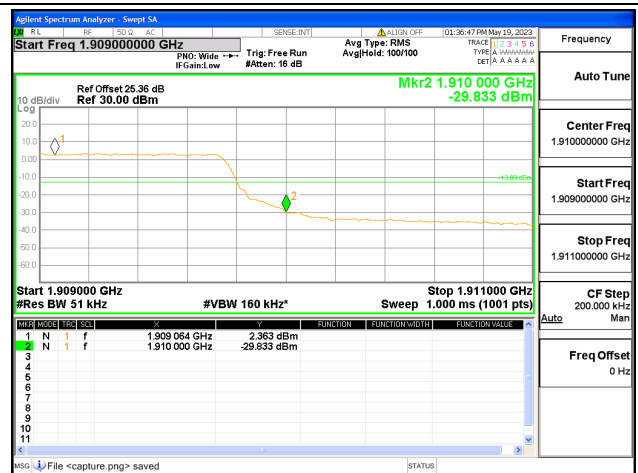
Band2 / 5MHz / High CH / QPSK / FULL RB
