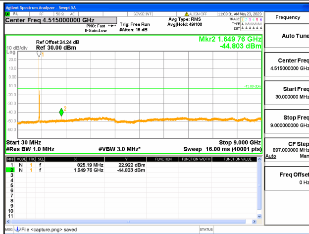
Band26 Part22 / 15MHz / Low CH / QPSK
