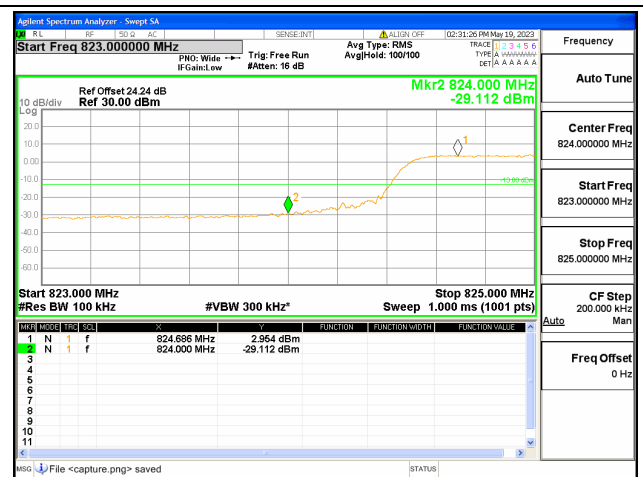
Band5 / 10MHz / Low CH / QPSK / FULL RB
