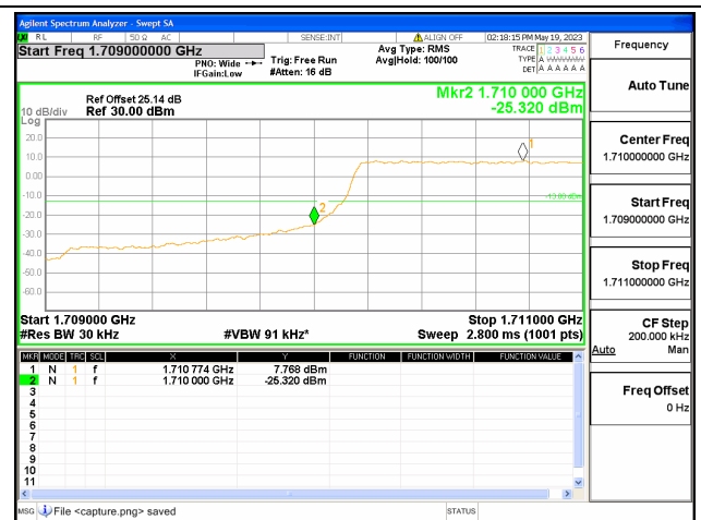
Band4 / 1.4MHz / Low CH / QPSK / FULL RB
