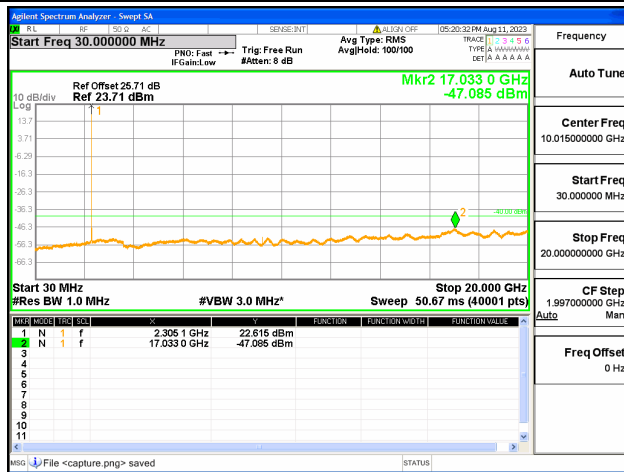
B30-30M-20G / 10MHz / Mid CH / QPSK
