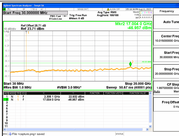
B30-30M-20G / 5MHz / Low CH / QPSK
