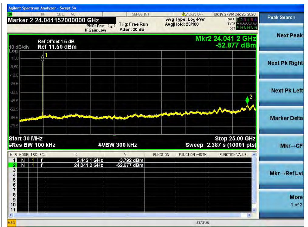
(30MHz to 25GHz, Channel 39, 8-DPSK)
