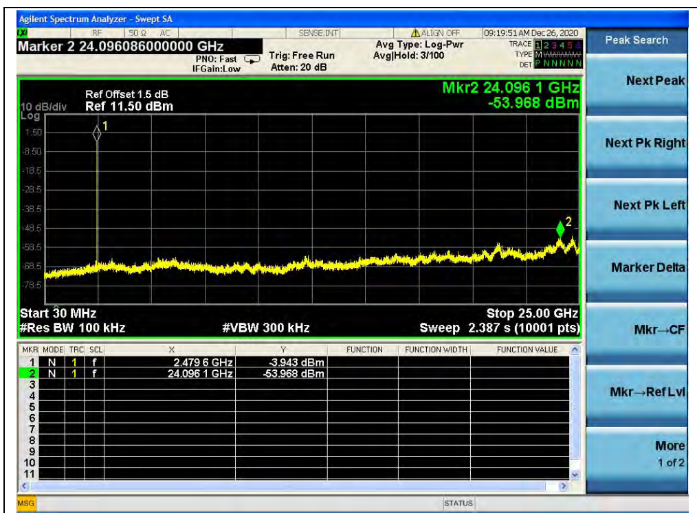
(30MHz to 25GHz, Channel 78, 8-DPSK)
