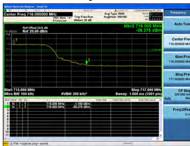
Band17 / 10MHz / High CH / QPSK / FULL RB
