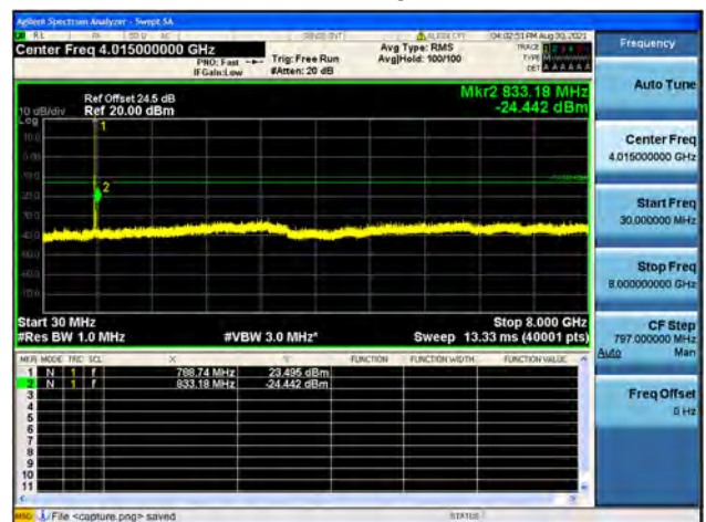
Band14 / 10MHz / High CH / 64QAM
