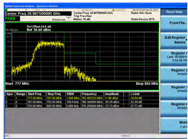
Band13 / 5MHz / High CH / QPSK / FULL RB
