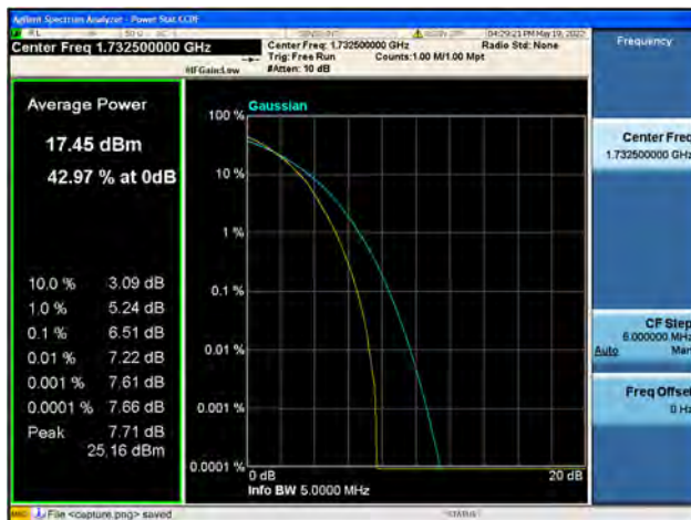
Band4 / 5MHz / Mid CH / 64QAM
