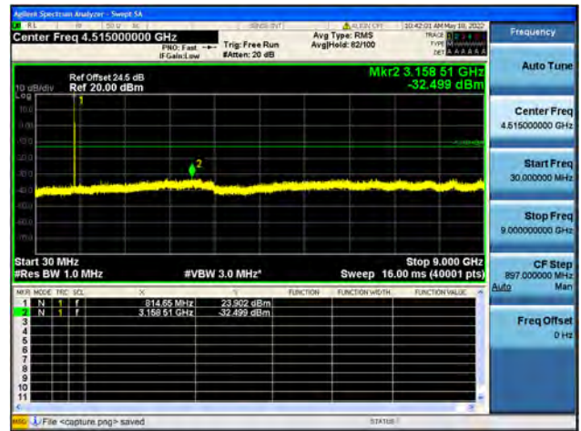
Band26 / 3MHz / Low CH / QPSK
