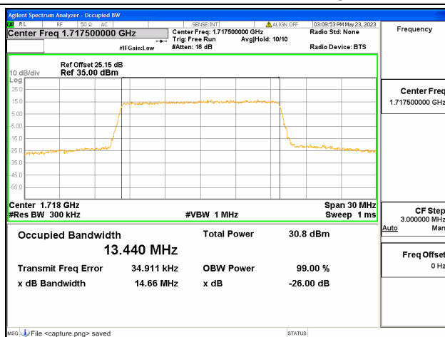
Band66 / 15MHz / QPSK/ Low CH
