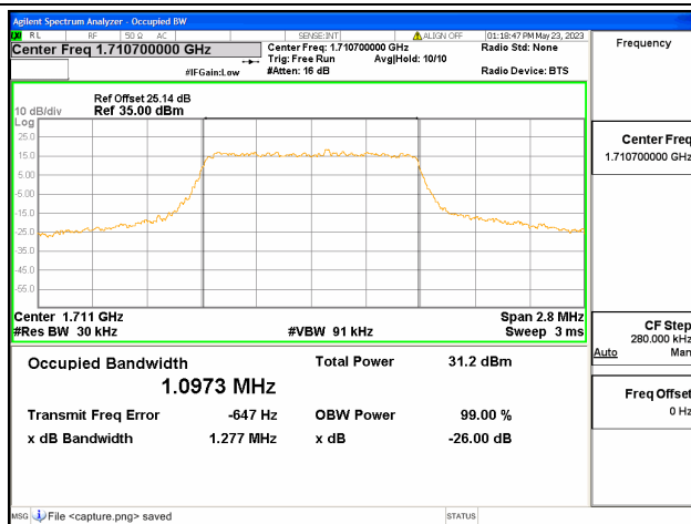
Band66 / 1.4MHz / QPSK/ Low CH
