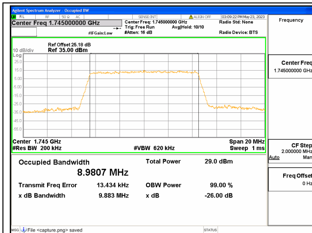
Band66 / 10MHz / 64QAM/ Mid CH
