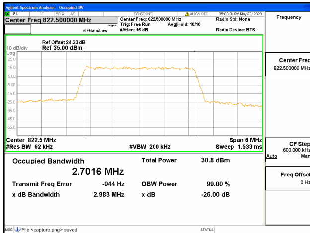
Band26 Part90 / 3MHz / 16QAM/ High CH
