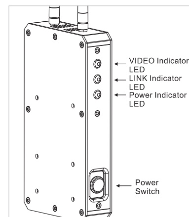
Operation Panel
