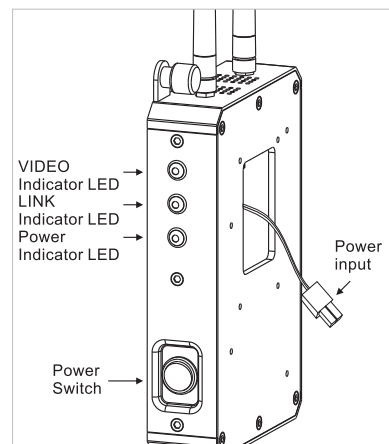
Operation Panel
