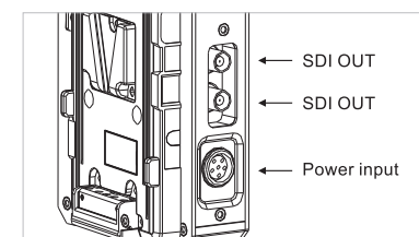
Back Panel
