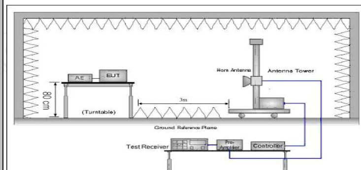
Above 1GHz
