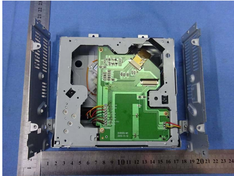
DVD echanism & Connect Board
