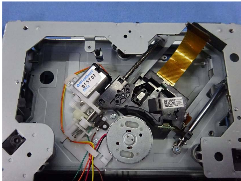
DVD echanism
