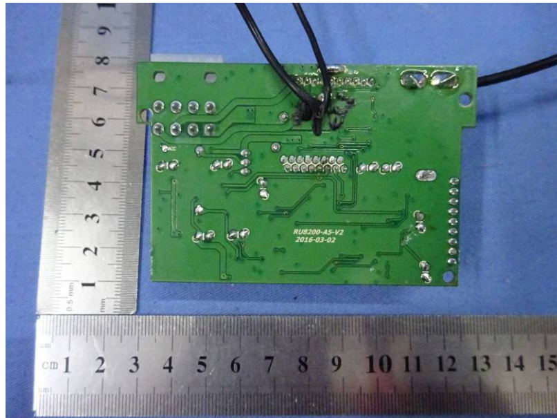
MAIN BOARD
