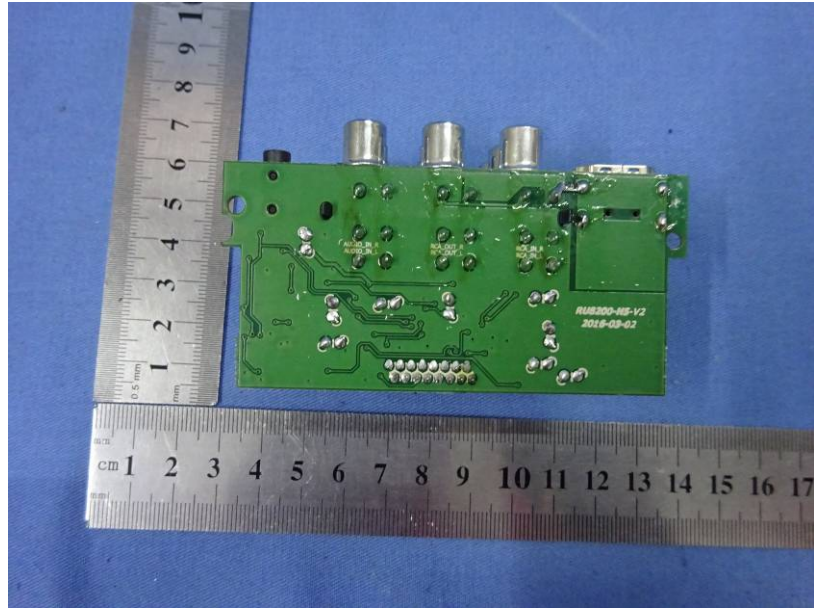
I/O BOARD
