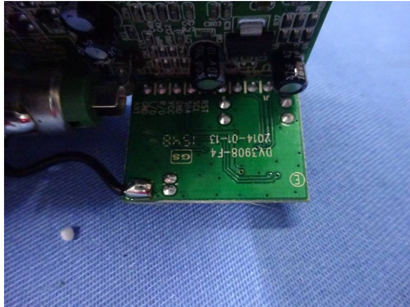
RECEIVE BOARD
