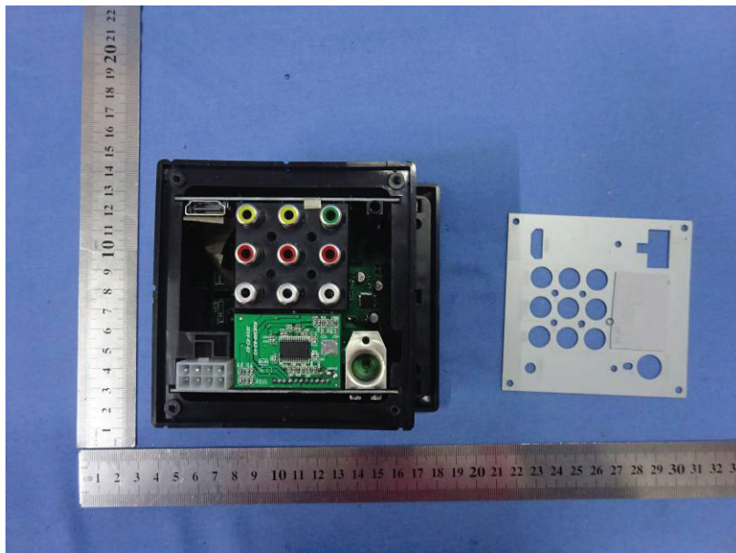
Uncover View
