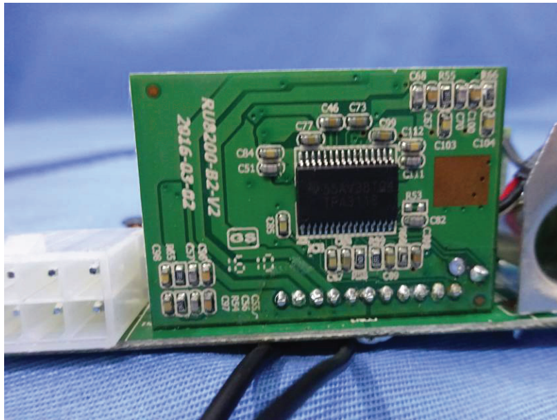
AMPLIFIER BOARD
