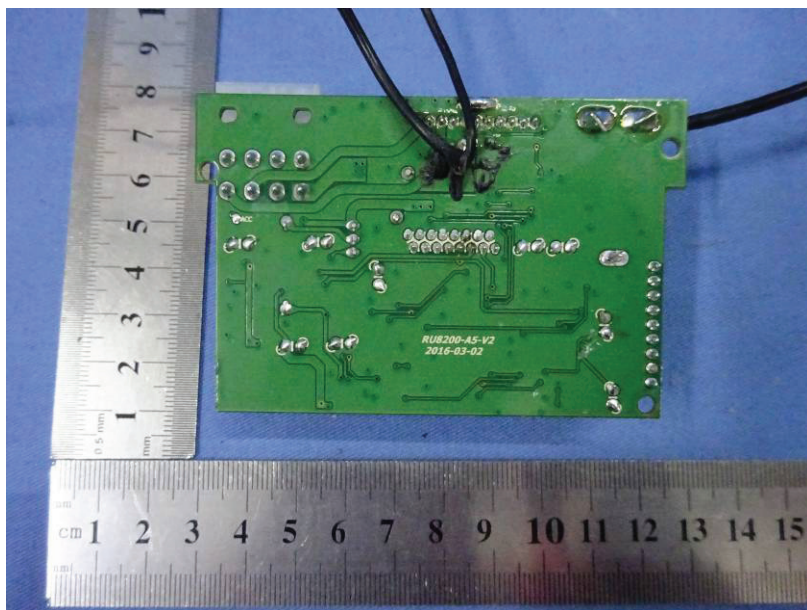
MAIN BOARD
