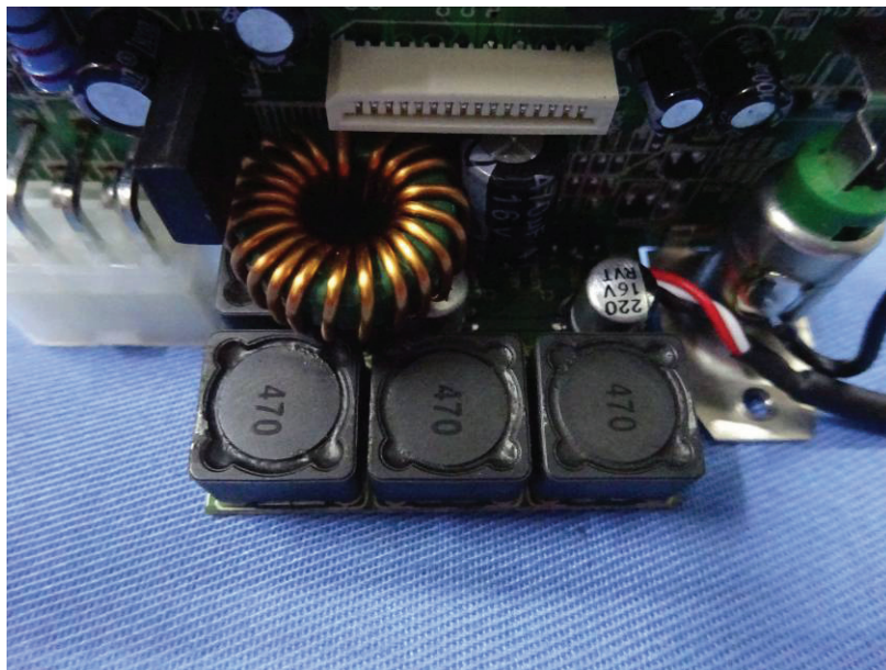
AMPLIFIER BOARD
