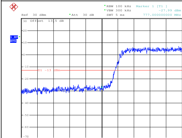
QPSK Low channel-25 RB offset 0
