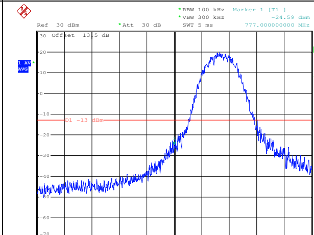
16QAM Low channel-25 RB offset 0
