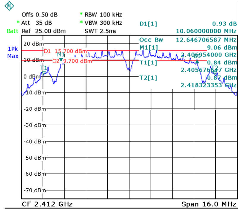
Low Channel
