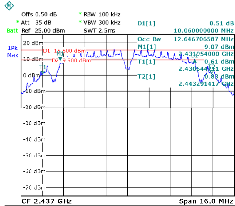
Middle Channel
