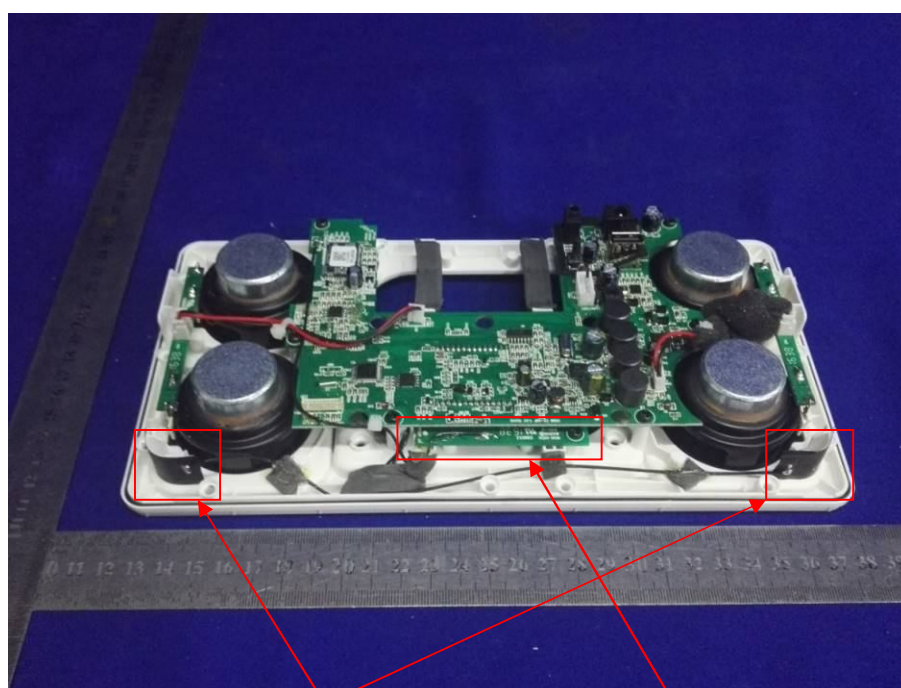
WIFI antenna
