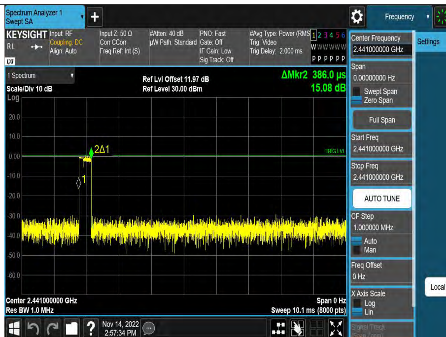
3DH1-Ant1-Hop-0.386-320
