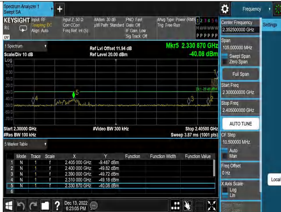
DH5-Ant1-Low-Hop_2402--9.49
