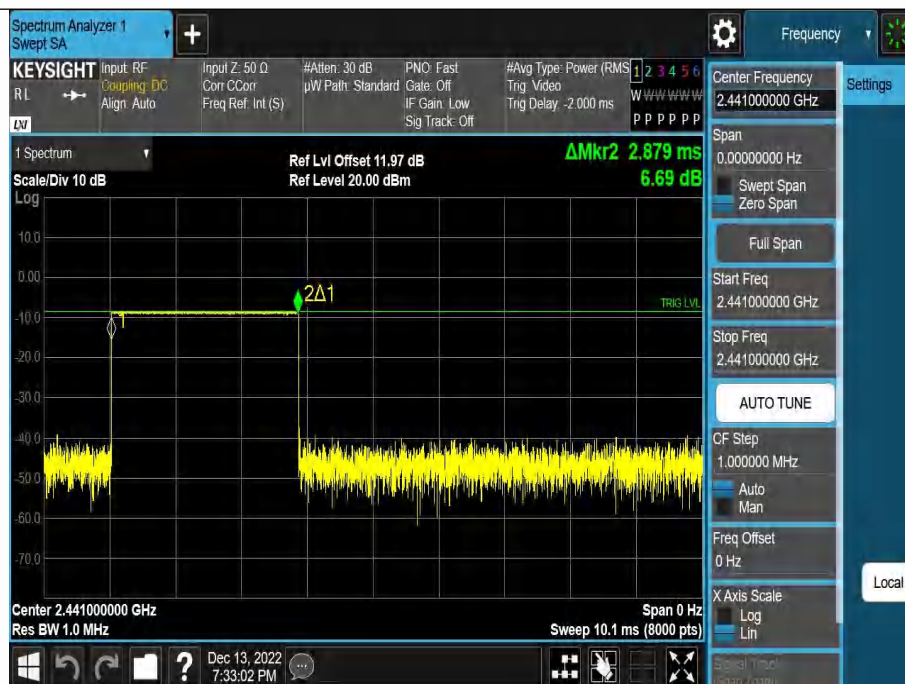
DH5-Ant1-Hop-2.879-106.67
