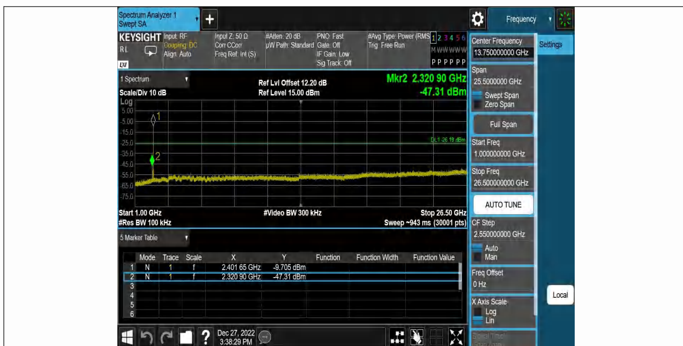
DH5-Ant1-2402-1000~26500--6.19
