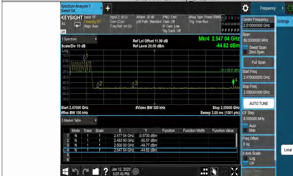
DH5-Ant1-High-Hop_2480--0.57
