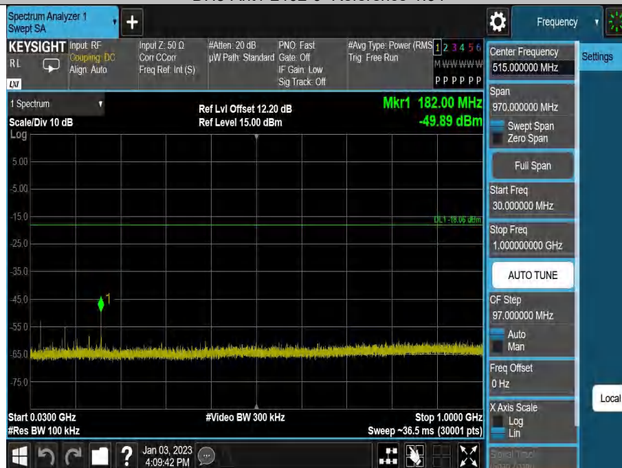
DH5-Ant1-2402-30~1000-1.94
