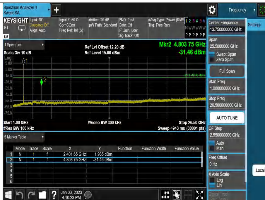
DH5-Ant1-2402-1000~26500-1.94
