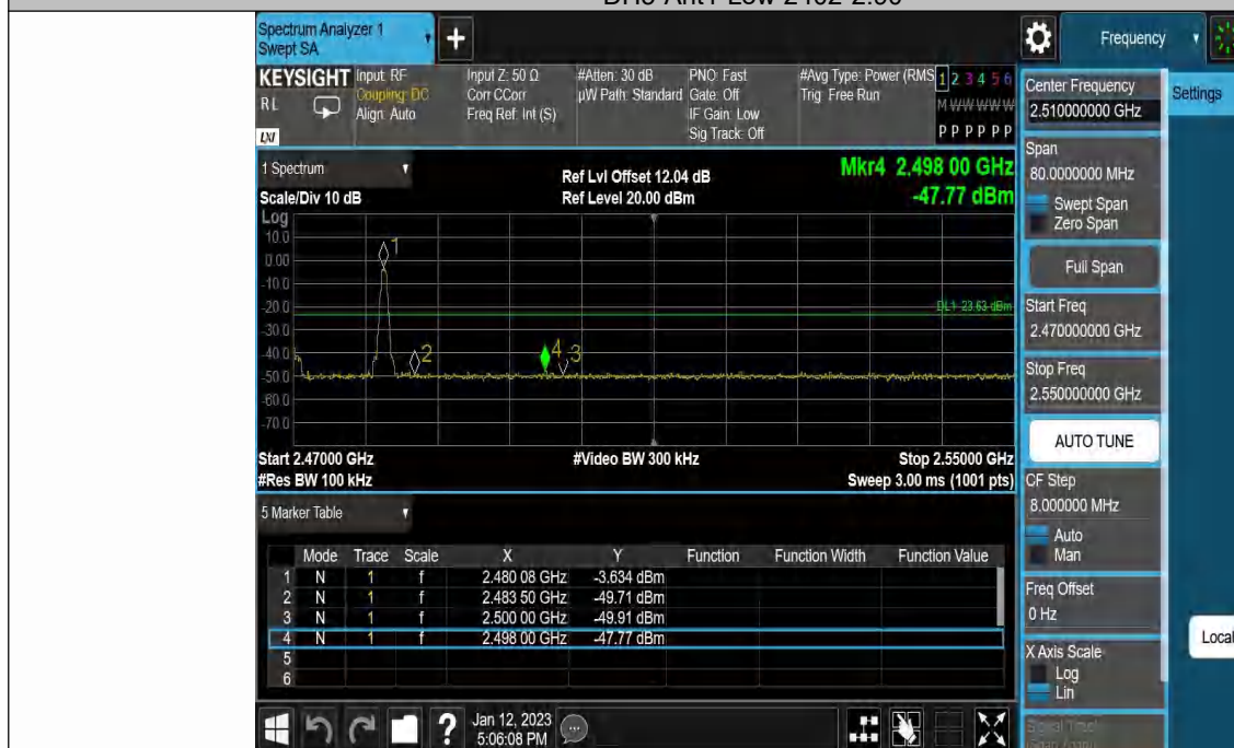
DH5-Ant1-High-2480--3.63
