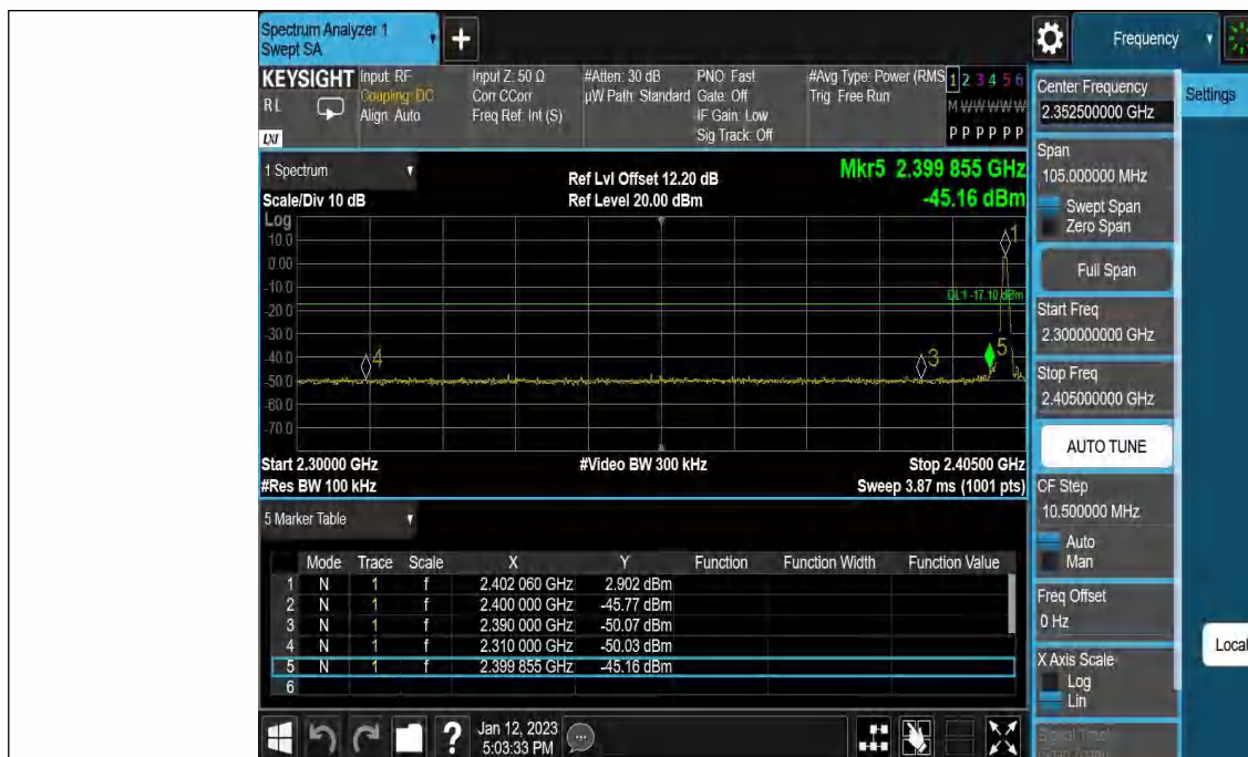
DH5-Ant1-Low-2402-2.90
