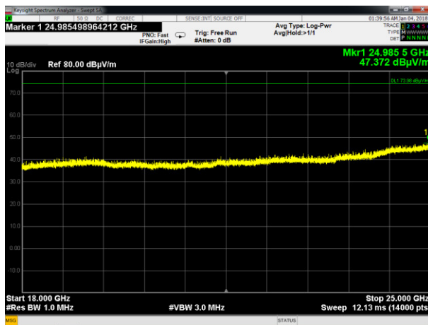
Plot 3.2.30: Radiated Emissions test, Horizontal Polarization, Tx Modulated, Field strength of harmonics, Cannel 39- Fc -2480, RC Base Station, CBS01, 18GHz -25GHz
