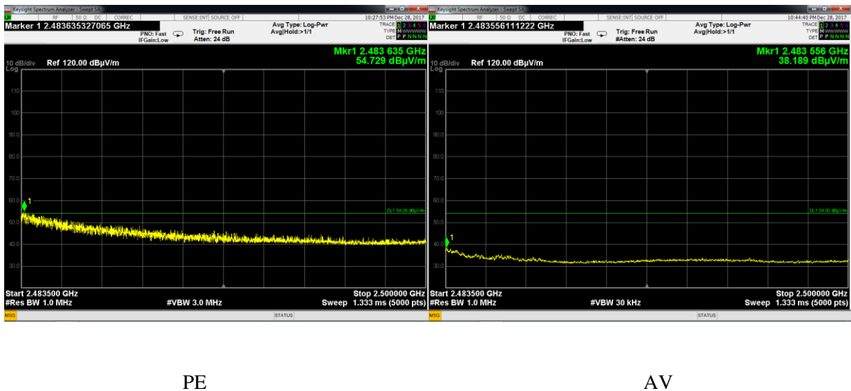
Plot 3.2.34: Radiated Emissions test, Horizontal Polarization, Tx Modulated, 2483.5MHz-2500MHz, Fc -2480
