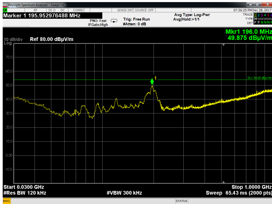
Plot 3.2.8: Radiated Emissions test, Horizontal Polarization, Tx Modulated, 30MHz-1GHz , Cannel 0- Fc -2402, RC Base Station, CBS01
