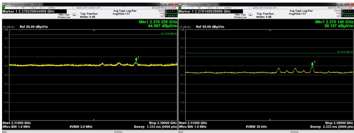
Plot 3.2.27: Radiated Emissions test, Horizontal Polarization, Tx Modulated, 2310MHz-2390MHz, Fc -2402, RX12
