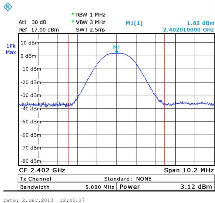
Figure 31 2402.00 MHz
