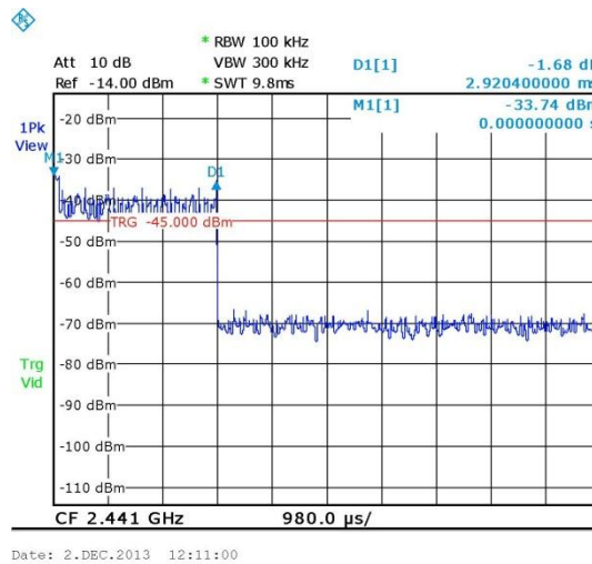
Figure 50. Avg. Factor – burst duration 2.92msec
