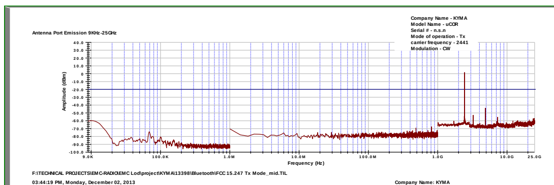
Figure 18 Spurious Conducted Emission – 2441 MHz
