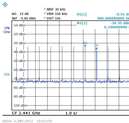
Figure 51. Avg. Factor – transmission within 100msec = 20\log(2.91/100) = -30.7\text{dB}
