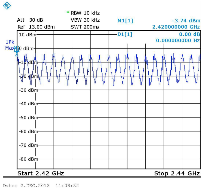
Figure 25. Frequency Hopping
