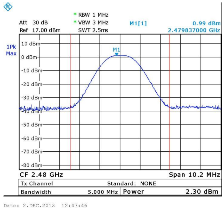
Figure 33 2480.00 MHz
